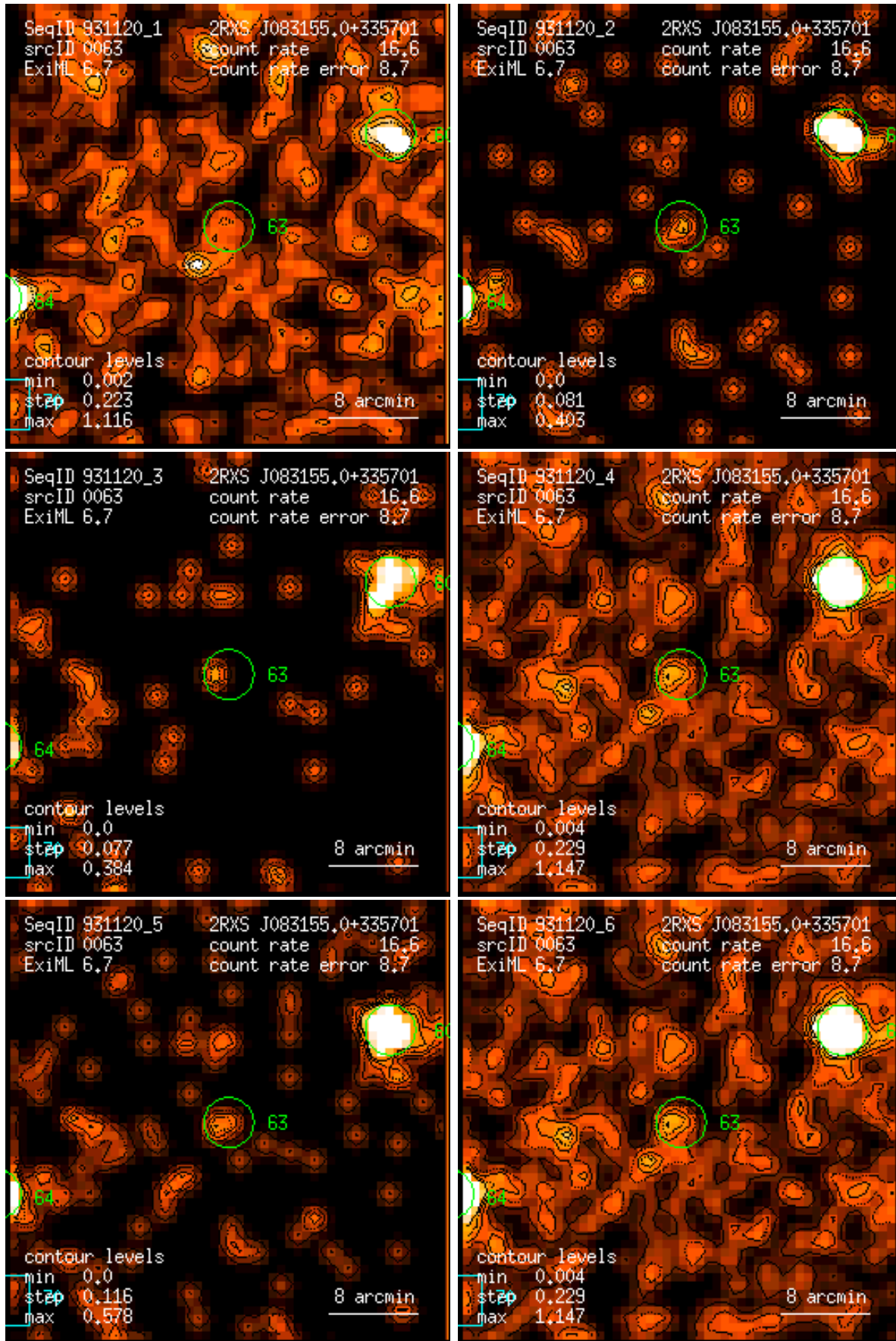
Figure 63: RASS 931120: detection 0063: band rate images, Gaussian filter: (1) PSPC channels 11 – 41, (2) 52 – 90, (3) 91 – 201, (4) 11 – 235, (5) 52 – 201, (6) 11 – 201. Broad band rates in counts/ks. Band rate contour levels in counts/ks/arcmin 2 .
