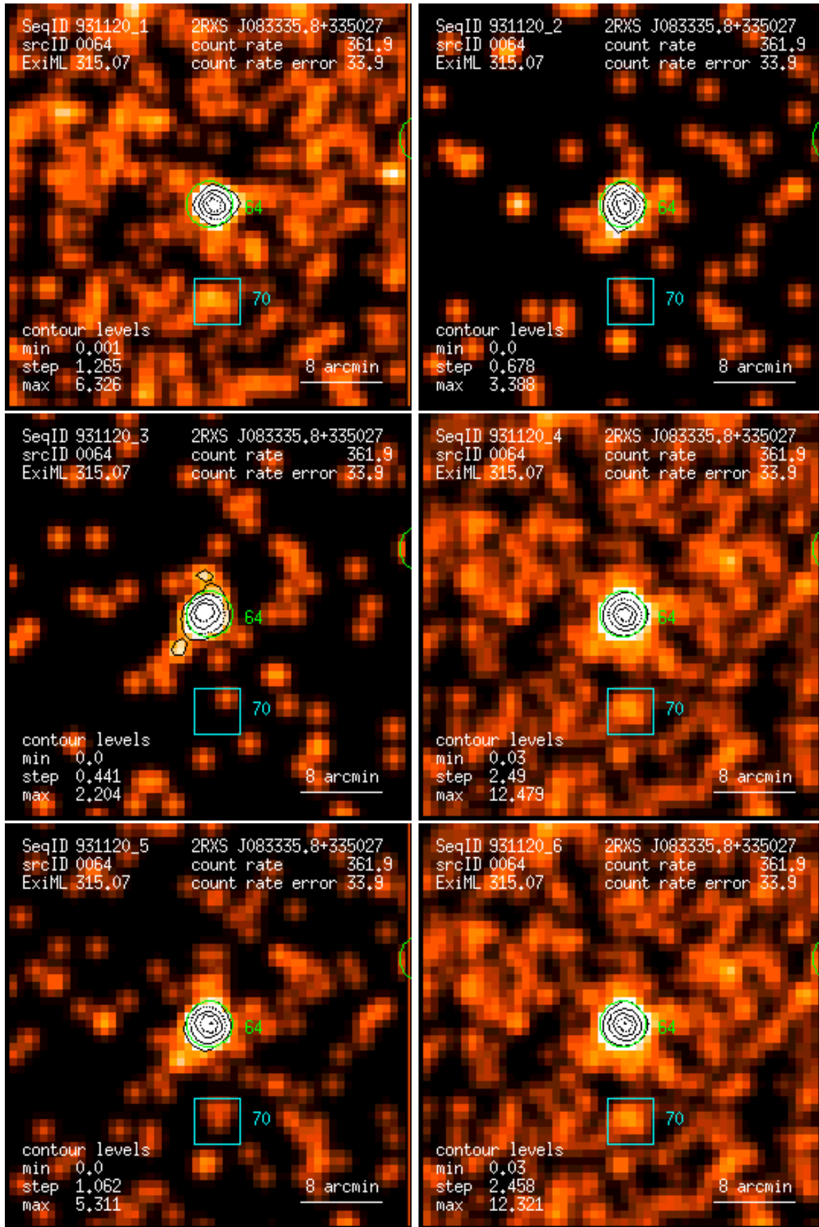
Figure 64: RASS 931120: detection 0064: band rate images, Gaussian filter: (1) PSPC channels 11 – 41, (2) 52 – 90, (3) 91 – 201, (4) 11 – 235, (5) 52 – 201, (6) 11 – 201. Broad band rates in counts/ks. Band rate contour levels in counts/ks/arcmin 2 .
