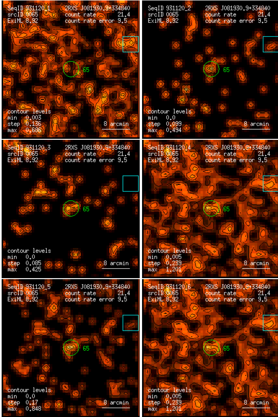
Figure 65: RASS 931120: detection 0065: band rate images, Gaussian filter: (1) PSPC channels 11 – 41, (2) 52 – 90, (3) 91 – 201, (4) 11 – 235, (5) 52 – 201, (6) 11 – 201. Broad band rates in counts/ks. Band rate contour levels in counts/ks/arcmin 2 .
