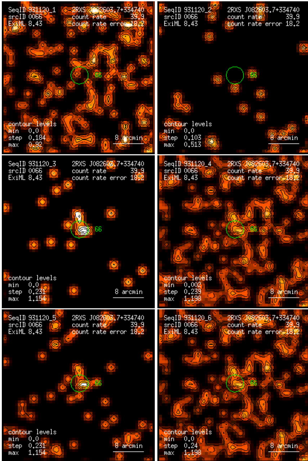
Figure 66: RASS 931120: detection 0066: band rate images, Gaussian filter: (1) PSPC channels 11 – 41, (2) 52 – 90, (3) 91 – 201, (4) 11 – 235, (5) 52 – 201, (6) 11 – 201. Broad band rates in counts/ks. Band rate contour levels in counts/ks/arcmin 2 .
