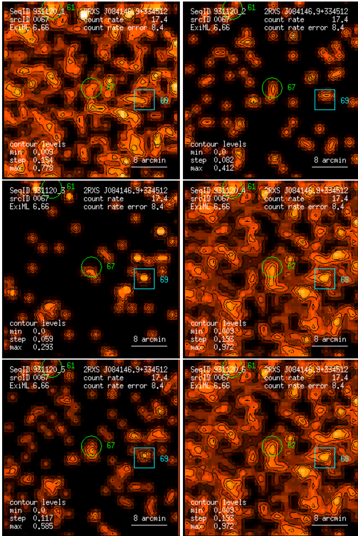
Figure 67: RASS 931120: detection 0067: band rate images, Gaussian filter: (1) PSPC channels 11 – 41, (2) 52 – 90, (3) 91 – 201, (4) 11 – 235, (5) 52 – 201, (6) 11 – 201. Broad band rates in counts/ks. Band rate contour levels in counts/ks/arcmin 2 .
