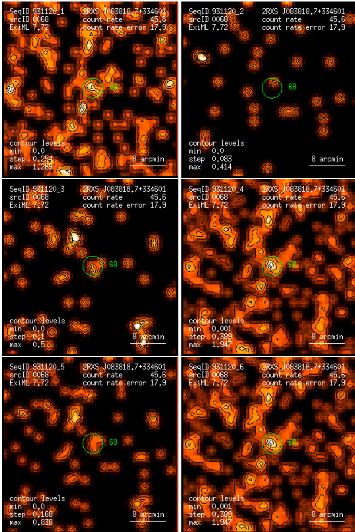
Figure 68: RASS 931120: detection 0068: band rate images, Gaussian filter: (1) PSPC channels 11 – 41, (2) 52 – 90, (3) 91 – 201, (4) 11 – 235, (5) 52 – 201, (6) 11 – 201. Broad band rates in counts/ks. Band rate contour levels in counts/ks/arcmin 2 .
