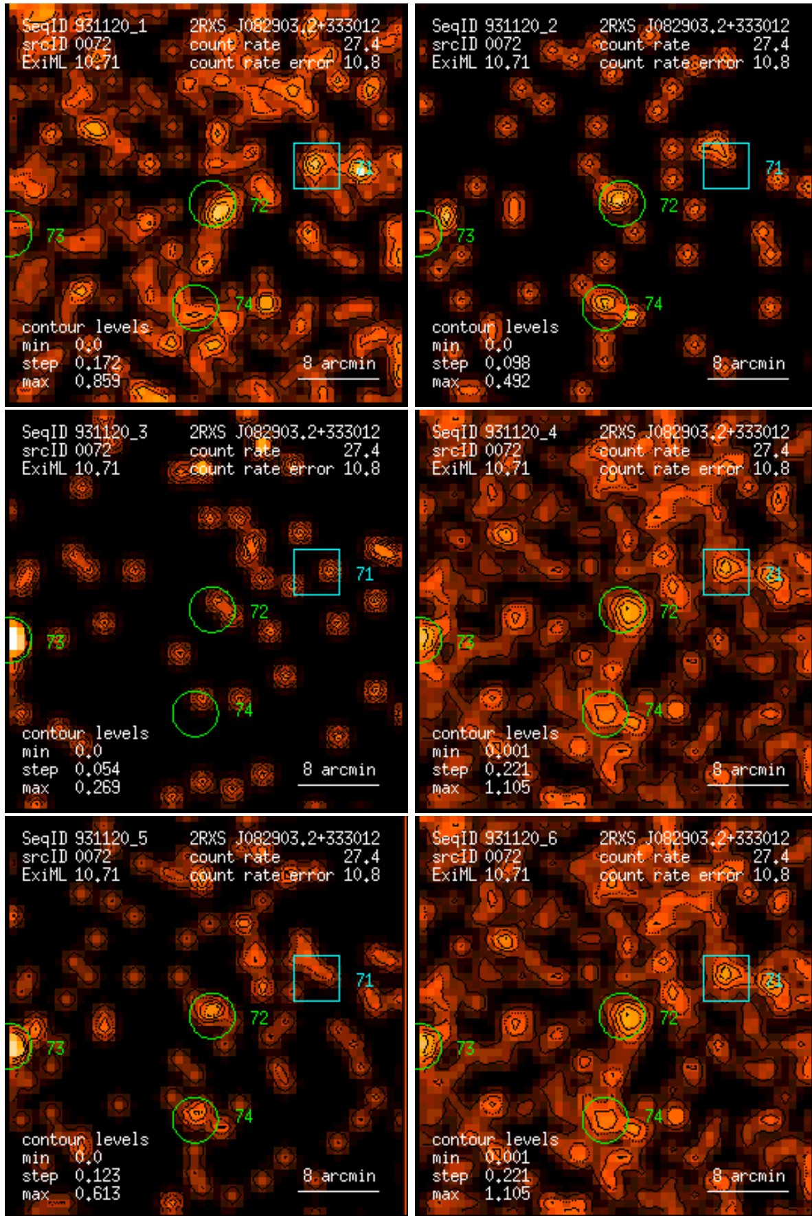
Figure 72: RASS 931120: detection 0072: band rate images, Gaussian filter: (1) PSPC channels 11 – 41, (2) 52 – 90, (3) 91 – 201, (4) 11 – 235, (5) 52 – 201, (6) 11 – 201. Broad band rates in counts/ks. Band rate contour levels in counts/ks/arcmin 2 .
