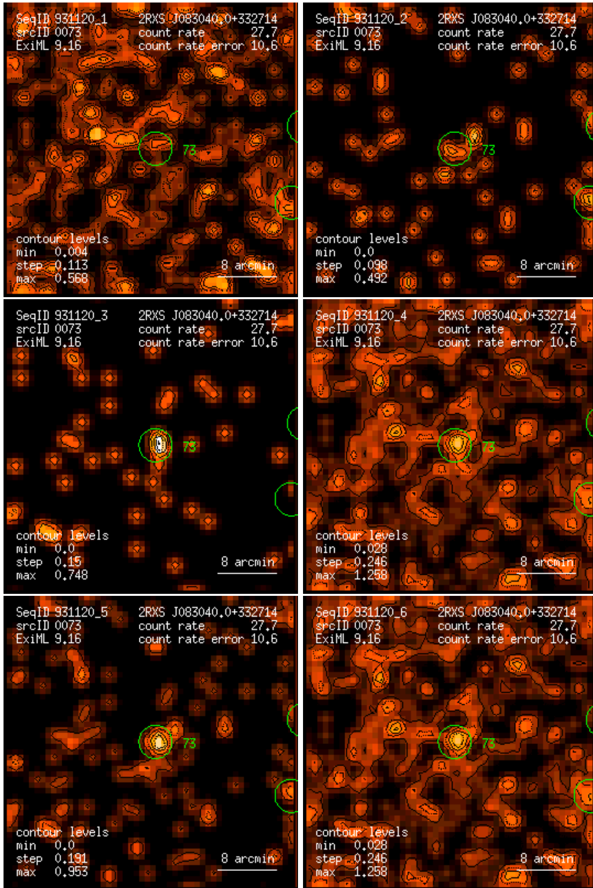
Figure 73: RASS 931120: detection 0073: band rate images, Gaussian filter: (1) PSPC channels 11 – 41, (2) 52 – 90, (3) 91 – 201, (4) 11 – 235, (5) 52 – 201, (6) 11 – 201. Broad band rates in counts/ks. Band rate contour levels in counts/ks/arcmin 2 .
