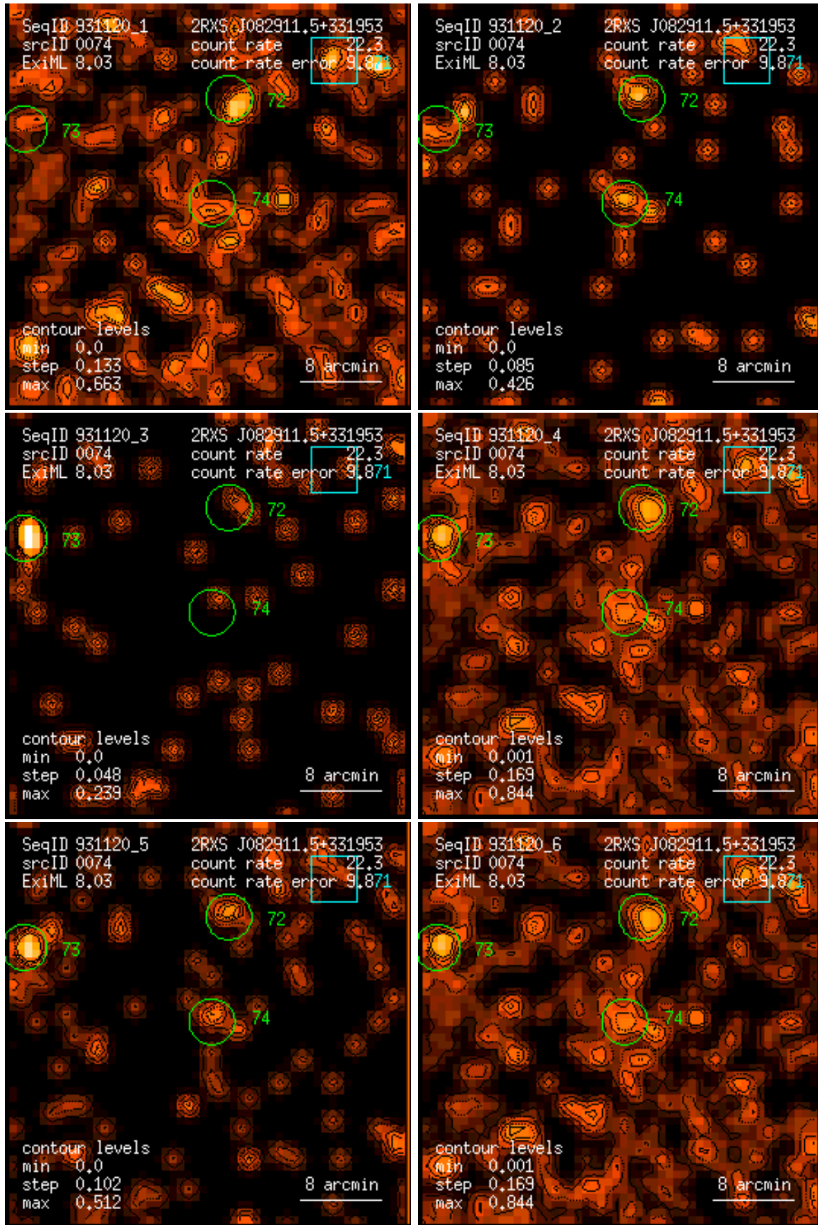
Figure 74: RASS 931120: detection 0074: band rate images, Gaussian filter: (1) PSPC channels 11 – 41, (2) 52 – 90, (3) 91 – 201, (4) 11 – 235, (5) 52 – 201, (6) 11 – 201. Broad band rates in counts/ks. Band rate contour levels in counts/ks/arcmin 2 .
