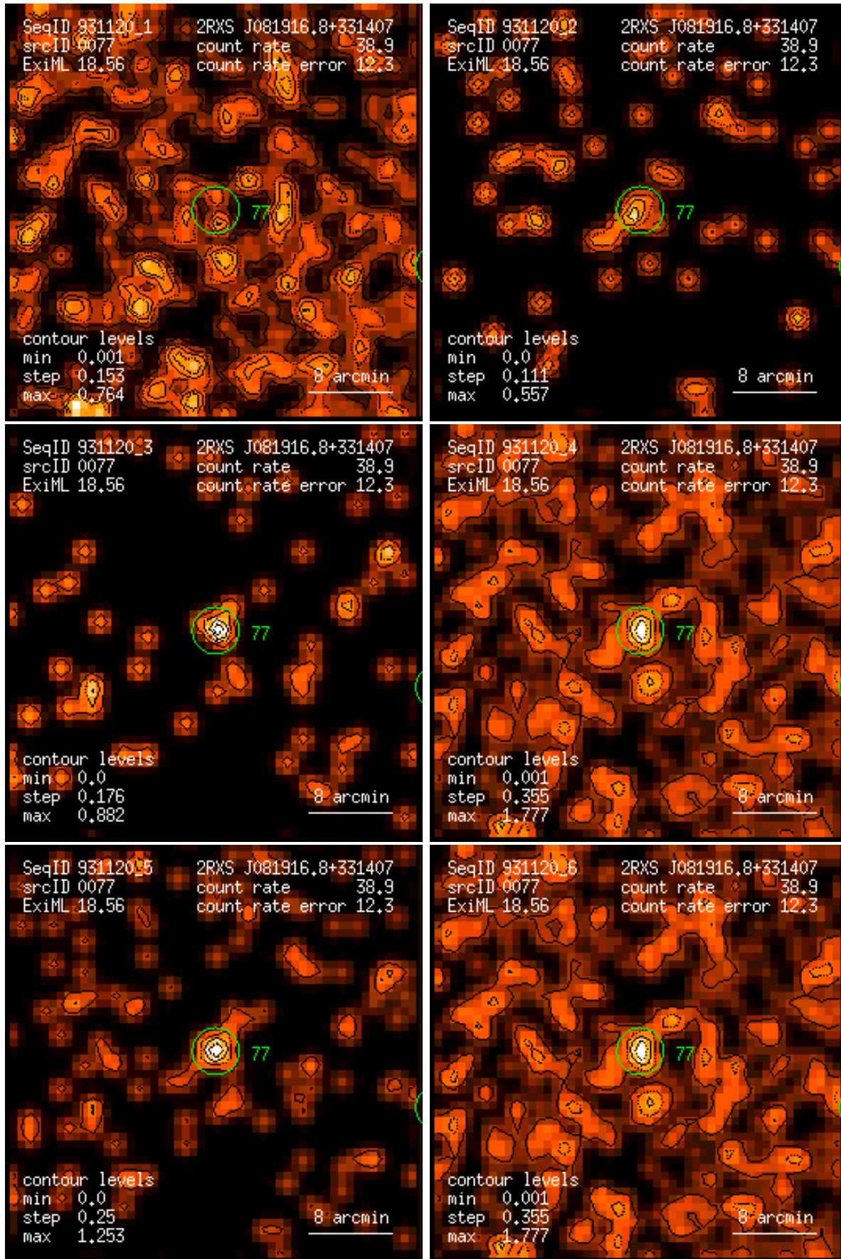
Figure 77: RASS 931120: detection 0077: band rate images, Gaussian filter: (1) PSPC channels 11 – 41, (2) 52 – 90, (3) 91 – 201, (4) 11 – 235, (5) 52 – 201, (6) 11 – 201. Broad band rates in counts/ks. Band rate contour levels in counts/ks/arcmin 2 .
