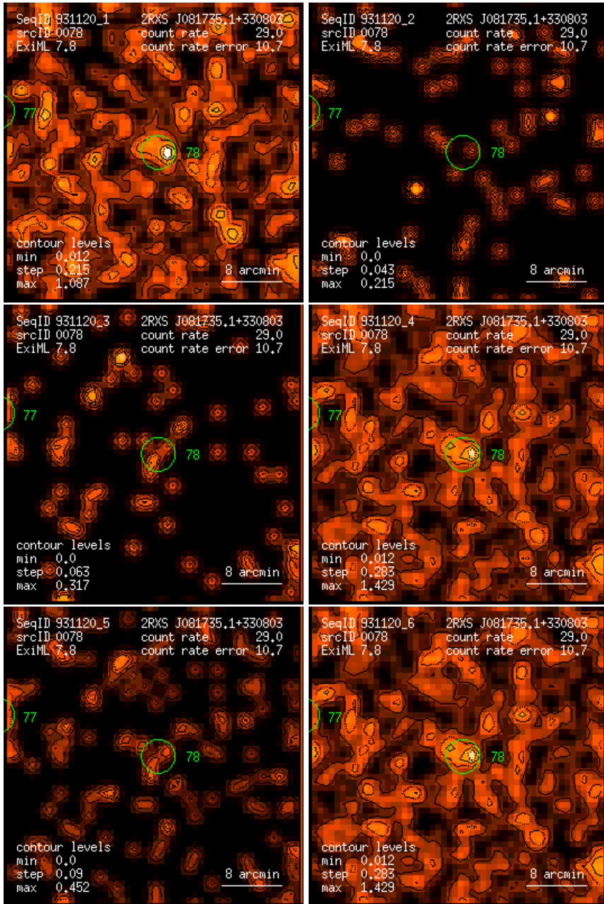
Figure 78: RASS 931120: detection 0078: band rate images, Gaussian filter: (1) PSPC channels 11 – 41, (2) 52 – 90, (3) 91 – 201, (4) 11 – 235, (5) 52 – 201, (6) 11 – 201. Broad band rates in counts/ks. Band rate contour levels in counts/ks/arcmin 2 .
