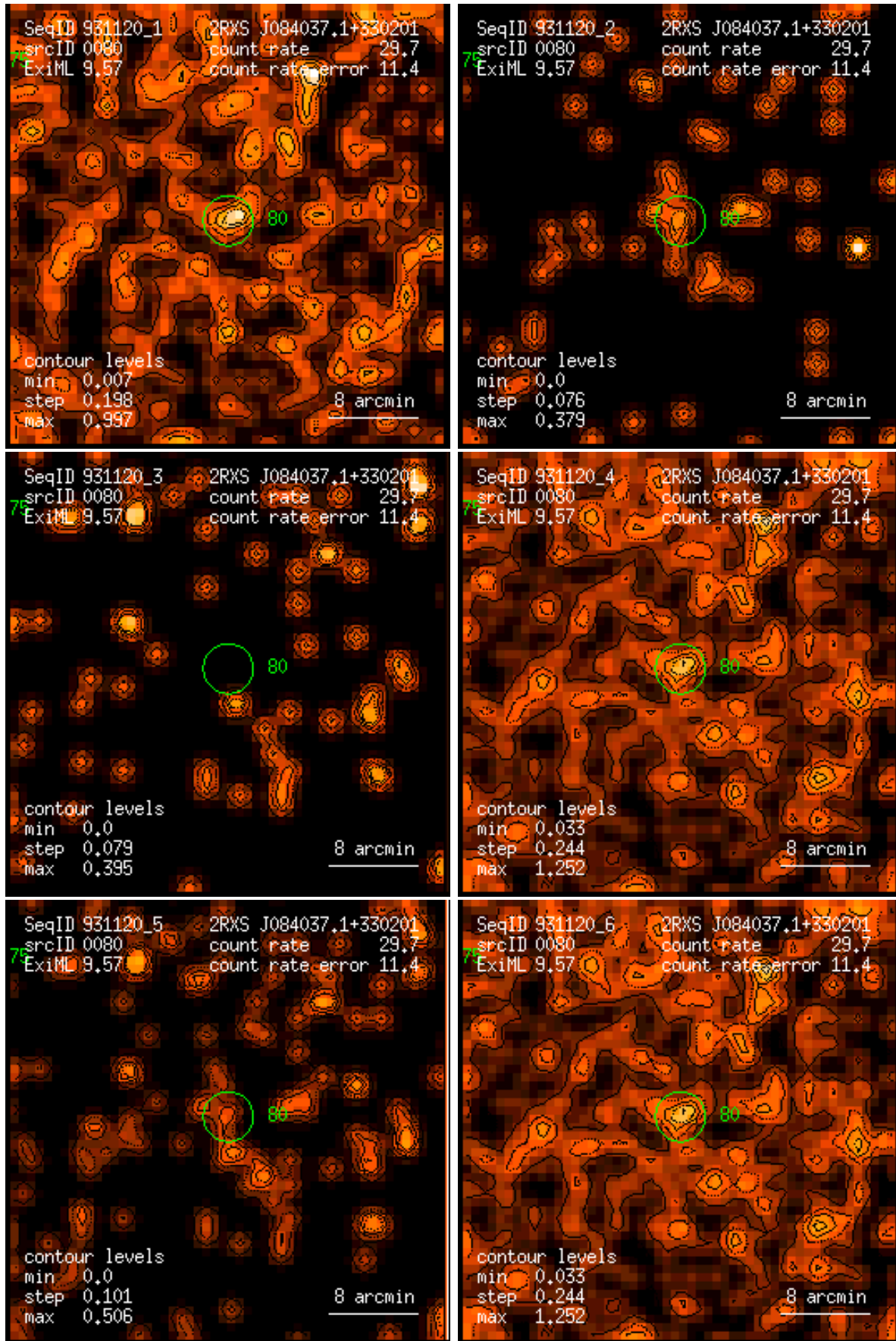
Figure 80: RASS 931120: detection 0080: band rate images, Gaussian filter: (1) PSPC channels 11 – 41, (2) 52 – 90, (3) 91 – 201, (4) 11 – 235, (5) 52 – 201, (6) 11 – 201. Broad band rates in counts/ks. Band rate contour levels in counts/ks/arcmin 2 .
