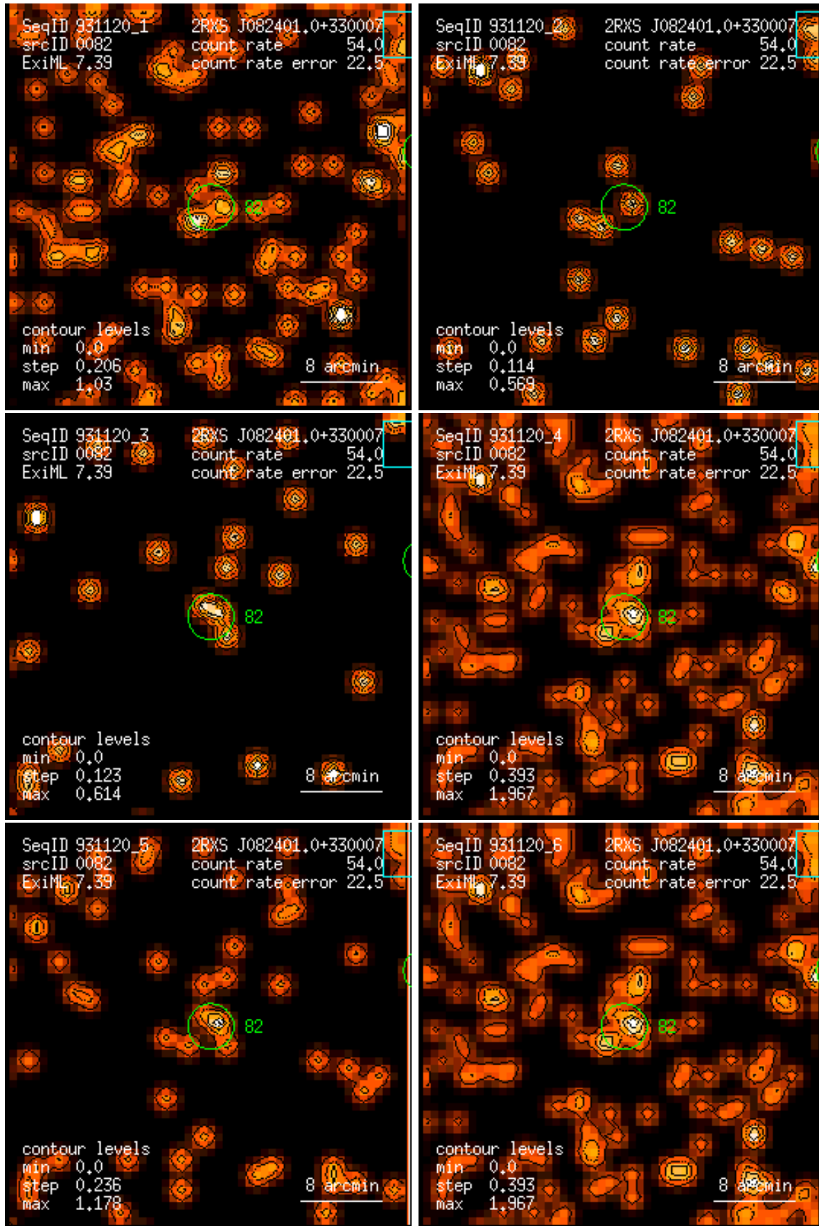
Figure 82: RASS 931120: detection 0082: band rate images, Gaussian filter: (1) PSPC channels 11 – 41, (2) 52 – 90, (3) 91 – 201, (4) 11 – 235, (5) 52 – 201, (6) 11 – 201. Broad band rates in counts/ks. Band rate contour levels in counts/ks/arcmin 2 .
