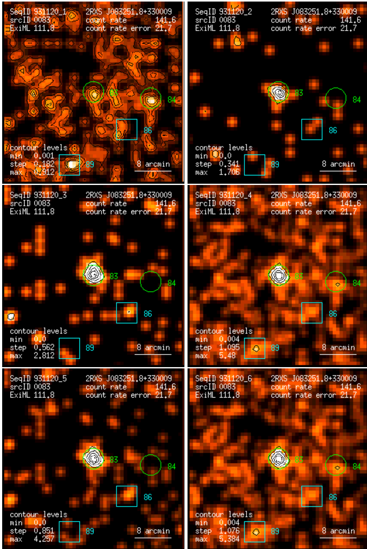
Figure 83: RASS 931120: detection 0083: band rate images, Gaussian filter: (1) PSPC channels 11 – 41, (2) 52 – 90, (3) 91 – 201, (4) 11 – 235, (5) 52 – 201, (6) 11 – 201. Broad band rates in counts/ks. Band rate contour levels in counts/ks/arcmin 2 .
