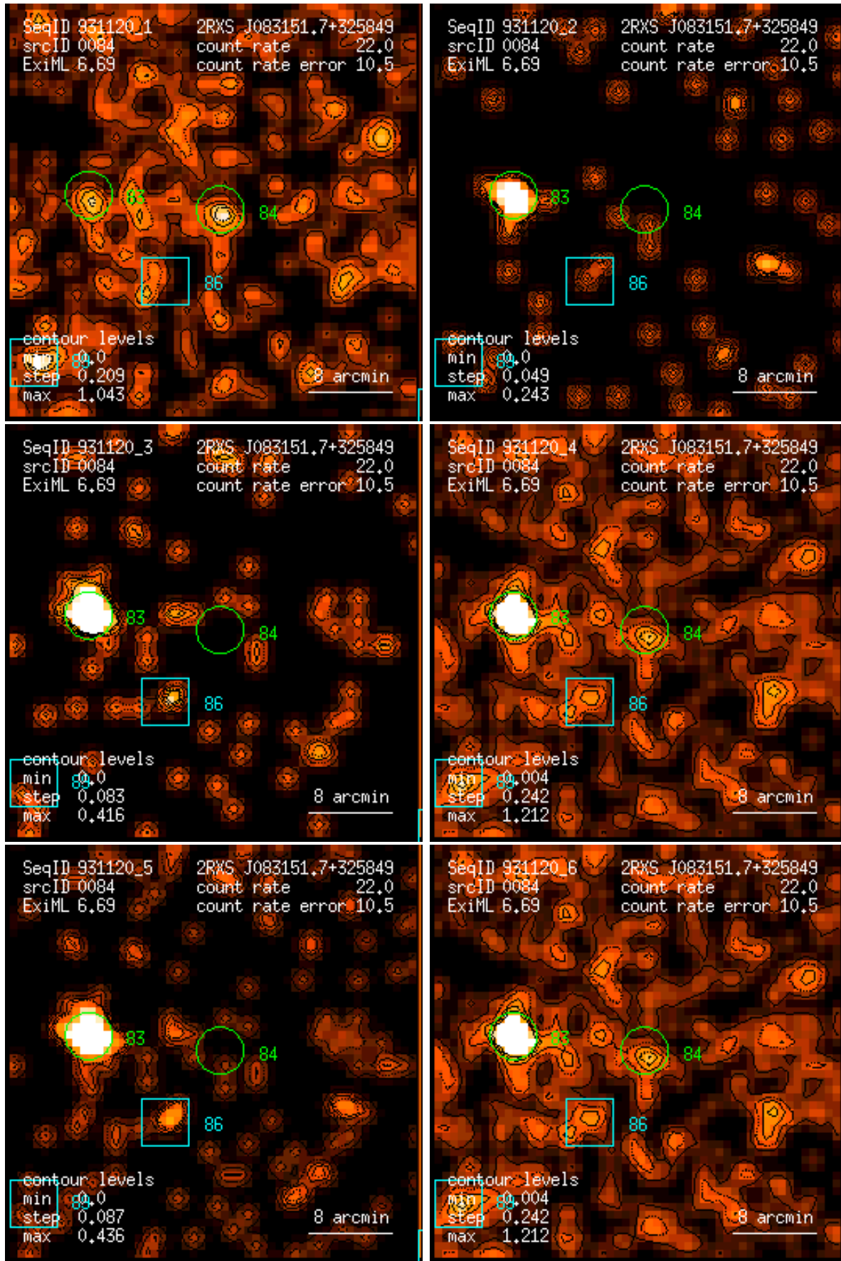
Figure 84: RASS 931120: detection 0084: band rate images, Gaussian filter: (1) PSPC channels 11 – 41, (2) 52 – 90, (3) 91 – 201, (4) 11 – 235, (5) 52 – 201, (6) 11 – 201. Broad band rates in counts/ks. Band rate contour levels in counts/ks/arcmin 2 .
