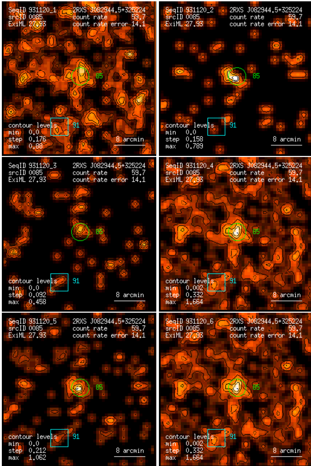
Figure 85: RASS 931120: detection 0085: band rate images, Gaussian filter: (1) PSPC channels 11 – 41, (2) 52 – 90, (3) 91 – 201, (4) 11 – 235, (5) 52 – 201, (6) 11 – 201. Broad band rates in counts/ks. Band rate contour levels in counts/ks/arcmin 2 .
