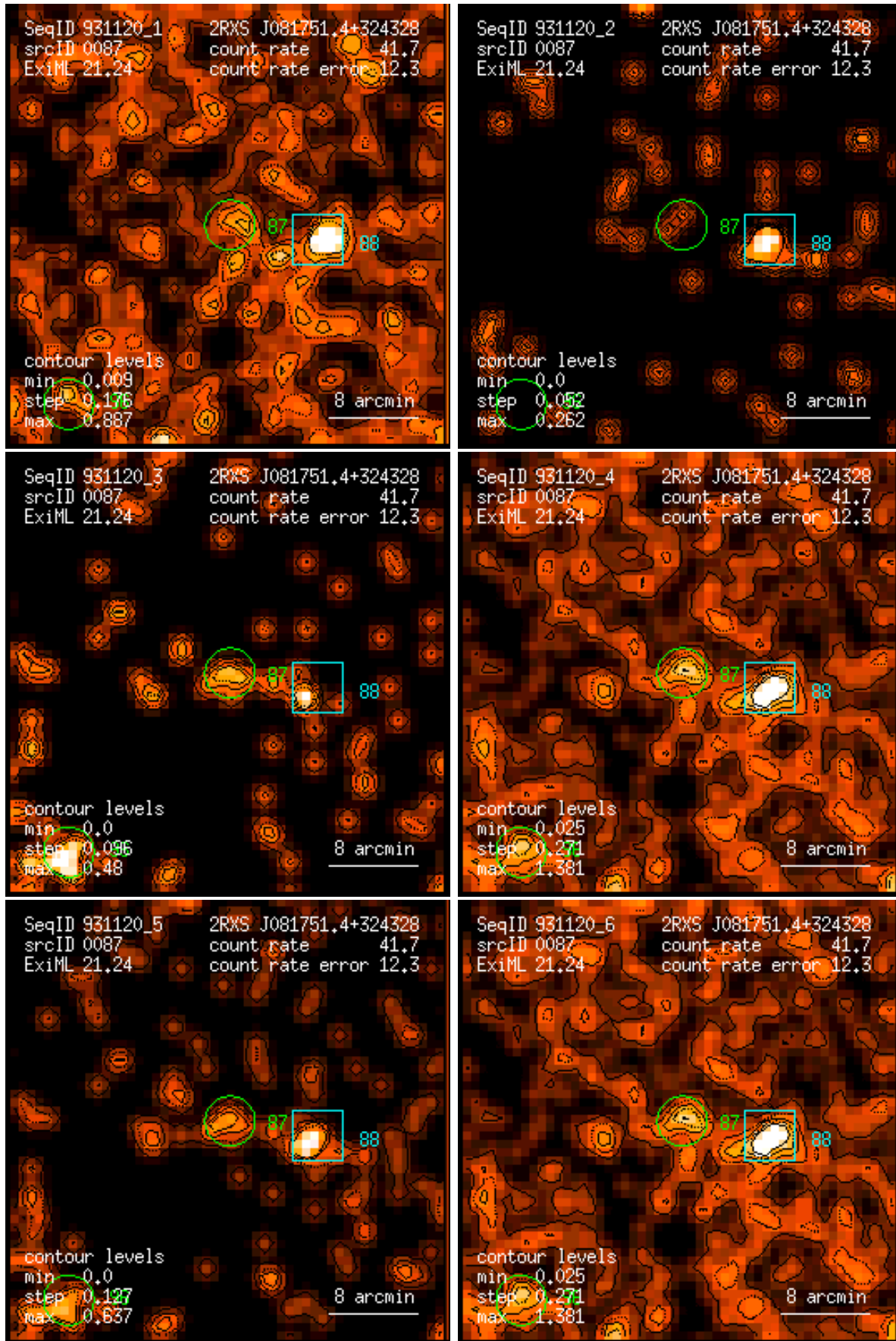
Figure 87: RASS 931120: detection 0087: band rate images, Gaussian filter: (1) PSPC channels 11 – 41, (2) 52 – 90, (3) 91 – 201, (4) 11 – 235, (5) 52 – 201, (6) 11 – 201. Broad band rates in counts/ks. Band rate contour levels in counts/ks/arcmin 2 .
