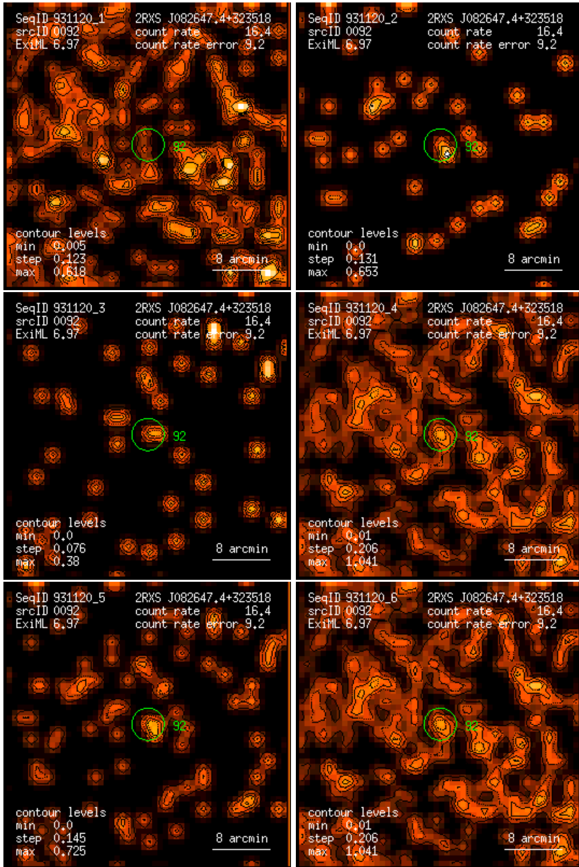
Figure 92: RASS 931120: detection 0092: band rate images, Gaussian filter: (1) PSPC channels 11 – 41, (2) 52 – 90, (3) 91 – 201, (4) 11 – 235, (5) 52 – 201, (6) 11 – 201. Broad band rates in counts/ks. Band rate contour levels in counts/ks/arcmin 2 .
