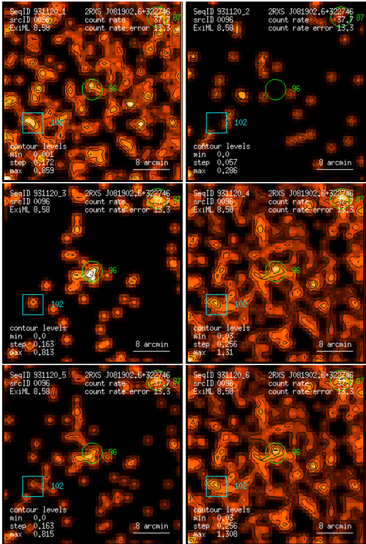
Figure 96: RASS 931120: detection 0096: band rate images, Gaussian filter: (1) PSPC channels 11 – 41, (2) 52 – 90, (3) 91 – 201, (4) 11 – 235, (5) 52 – 201, (6) 11 – 201. Broad band rates in counts/ks. Band rate contour levels in counts/ks/arcmin 2 .
