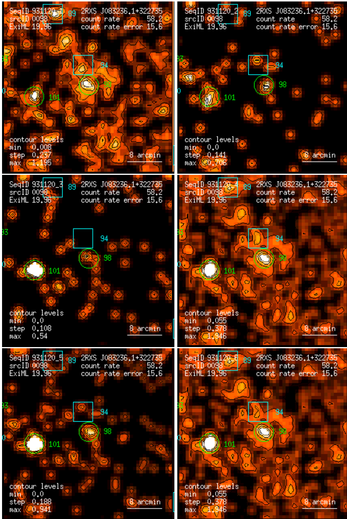
Figure 98: RASS 931120: detection 0098: band rate images, Gaussian filter: (1) PSPC channels 11 – 41, (2) 52 – 90, (3) 91 – 201, (4) 11 – 235, (5) 52 – 201, (6) 11 – 201. Broad band rates in counts/ks. Band rate contour levels in counts/ks/arcmin 2 .
