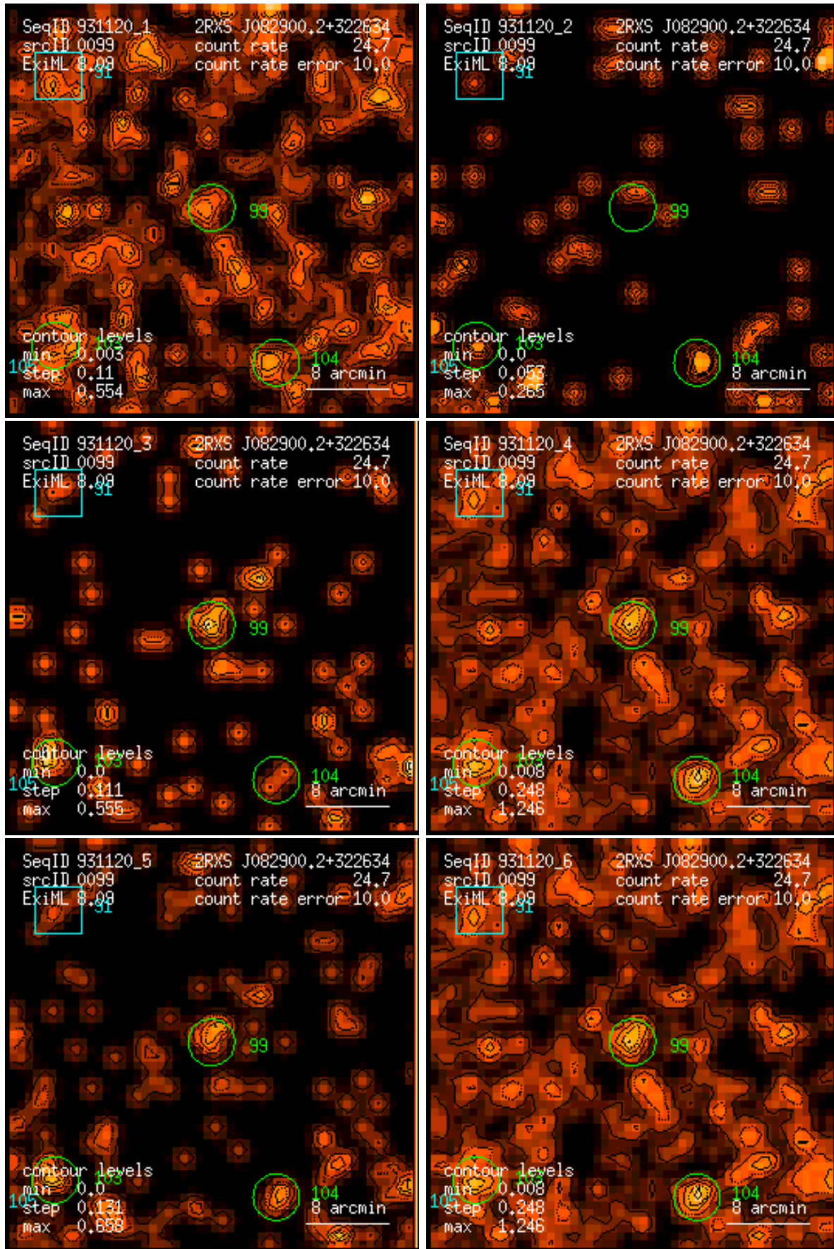
Figure 99: RASS 931120: detection 0099: band rate images, Gaussian filter: (1) PSPC channels 11 – 41, (2) 52 – 90, (3) 91 – 201, (4) 11 – 235, (5) 52 – 201, (6) 11 – 201. Broad band rates in counts/ks. Band rate contour levels in counts/ks/arcmin 2 .
