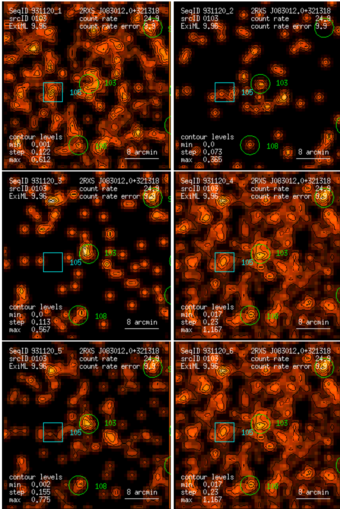
Figure 103: RASS 931120: detection 0103: band rate images, Gaussian filter: (1) PSPC channels 11 – 41, (2) 52 – 90, (3) 91 – 201, (4) 11 – 235, (5) 52 – 201, (6) 11 – 201. Broad band rates in counts/ks. Band rate contour levels in counts/ks/arcmin 2 .
