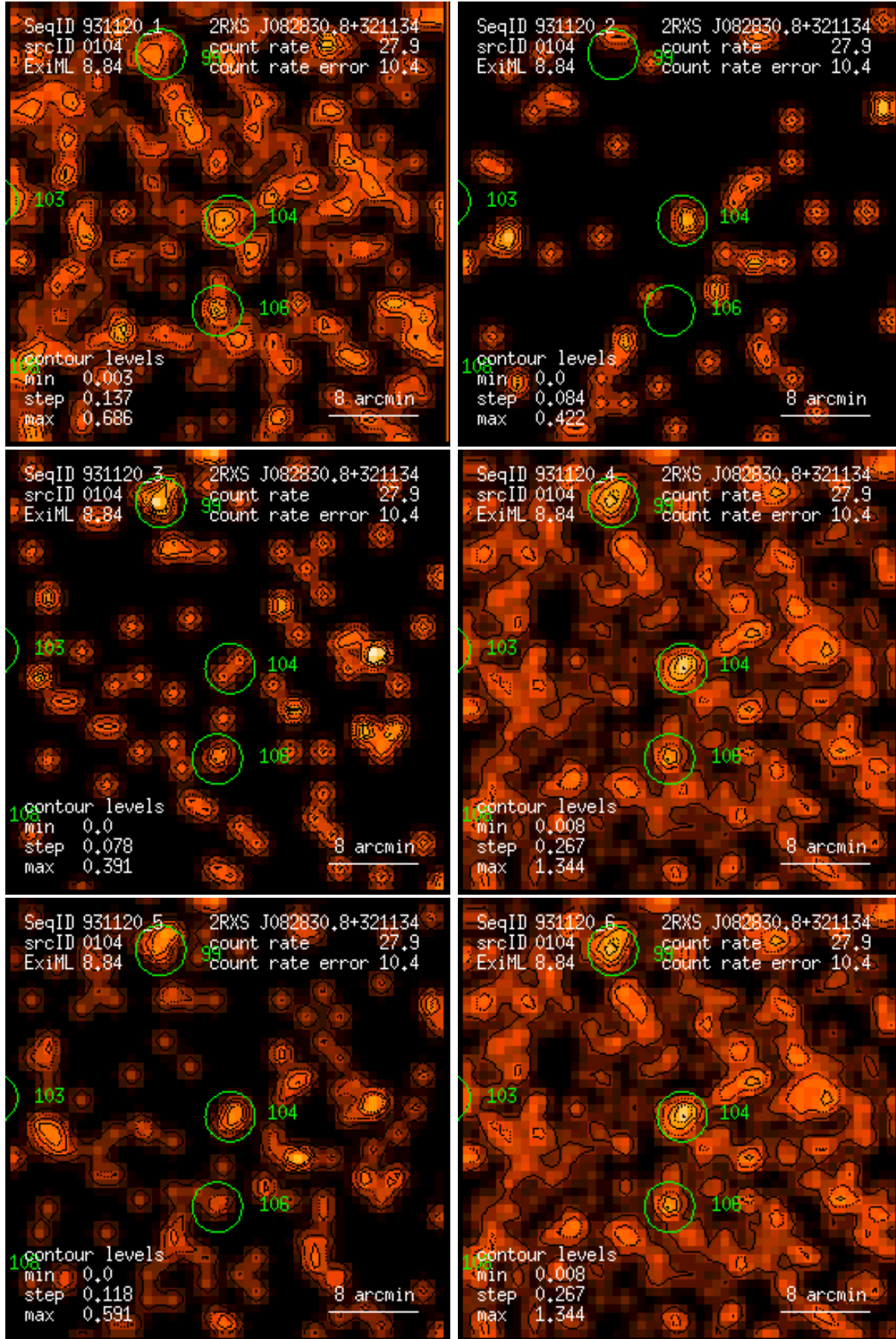
Figure 104: RASS 931120: detection 0104: band rate images, Gaussian filter: (1) PSPC channels 11 – 41, (2) 52 – 90, (3) 91 – 201, (4) 11 – 235, (5) 52 – 201, (6) 11 – 201. Broad band rates in counts/ks. Band rate contour levels in counts/ks/arcmin 2 .
