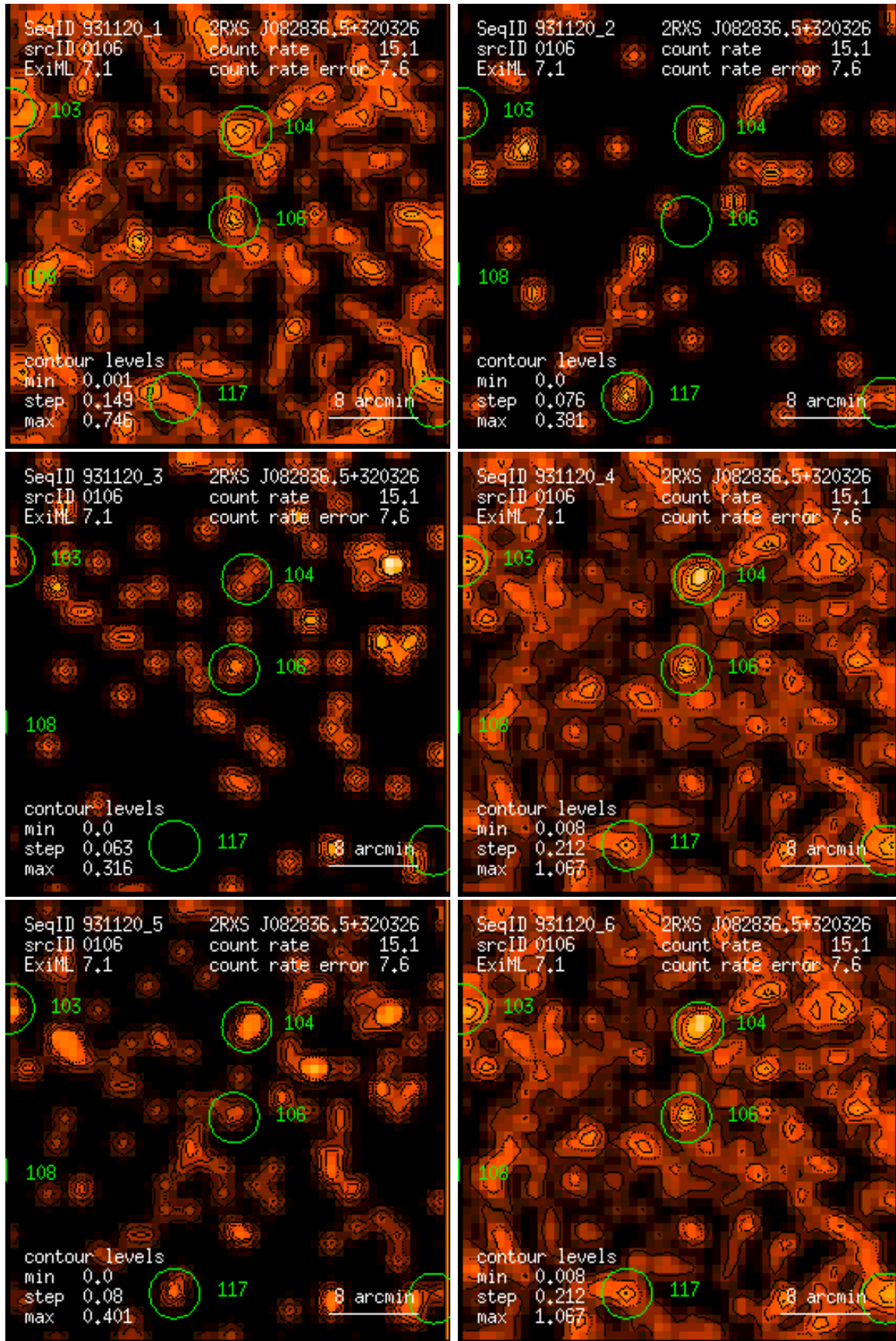
Figure 106: RASS 931120: detection 0106: band rate images, Gaussian filter: (1) PSPC channels 11 – 41, (2) 52 – 90, (3) 91 – 201, (4) 11 – 235, (5) 52 – 201, (6) 11 – 201. Broad band rates in counts/ks. Band rate contour levels in counts/ks/arcmin 2 .
