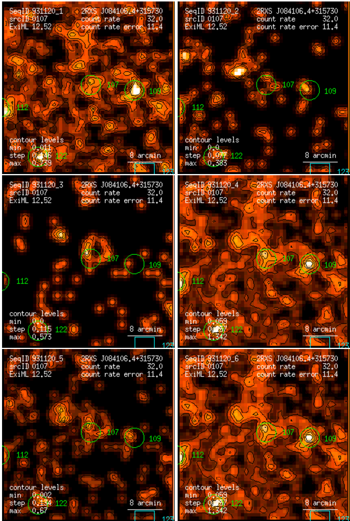
Figure 107: RASS 931120: detection 0107: band rate images, Gaussian filter: (1) PSPC channels 11 – 41, (2) 52 – 90, (3) 91 – 201, (4) 11 – 235, (5) 52 – 201, (6) 11 – 201. Broad band rates in counts/ks. Band rate contour levels in counts/ks/arcmin 2 .
