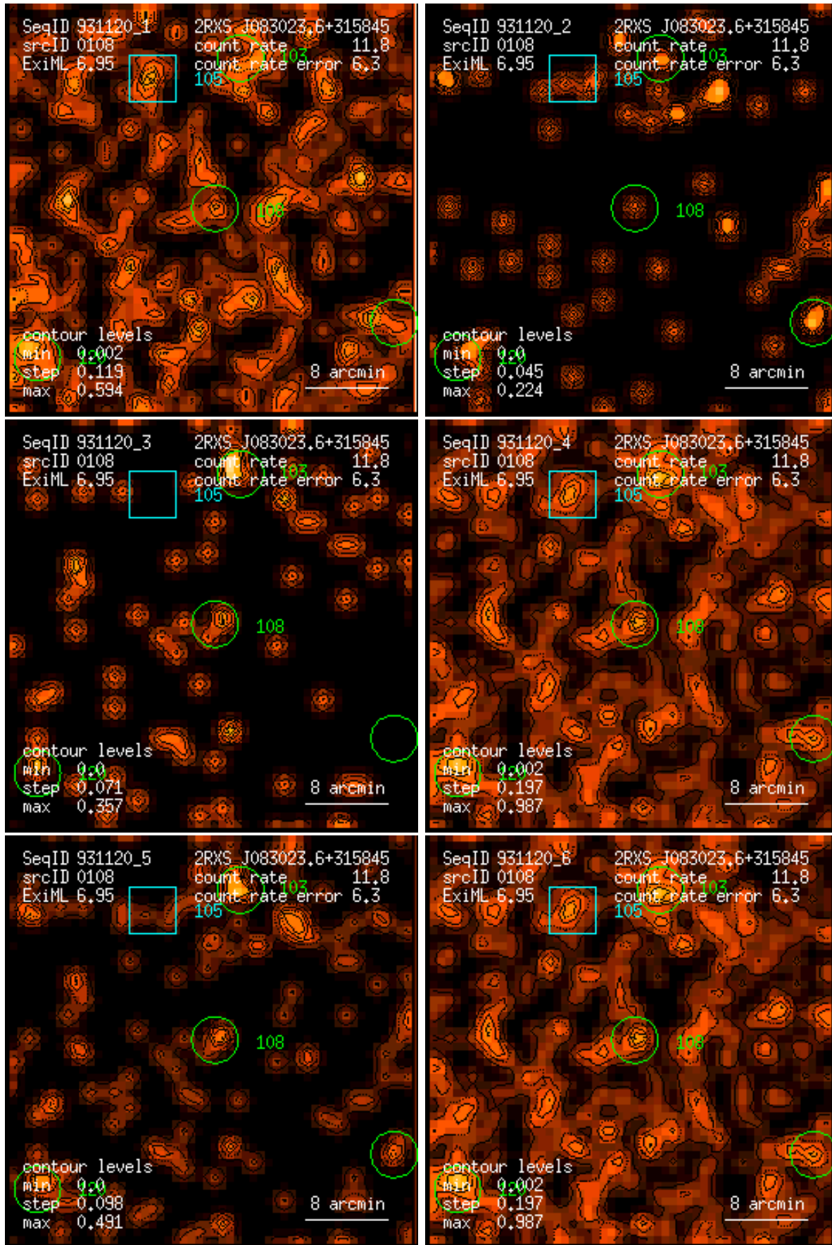
Figure 108: RASS 931120: detection 0108: band rate images, Gaussian filter: (1) PSPC channels 11 – 41, (2) 52 – 90, (3) 91 – 201, (4) 11 – 235, (5) 52 – 201, (6) 11 – 201. Broad band rates in counts/ks. Band rate contour levels in counts/ks/arcmin 2 .
