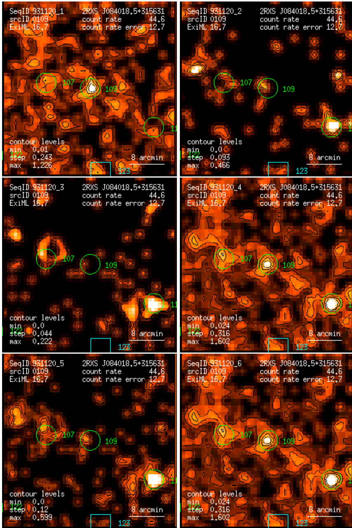
Figure 109: RASS 931120: detection 0109: band rate images, Gaussian filter: (1) PSPC channels 11 – 41, (2) 52 – 90, (3) 91 – 201, (4) 11 – 235, (5) 52 – 201, (6) 11 – 201. Broad band rates in counts/ks. Band rate contour levels in counts/ks/arcmin 2 .
