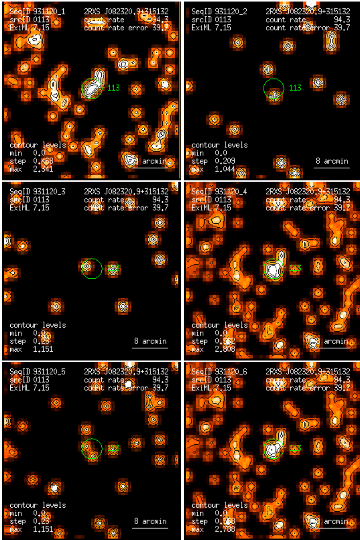
Figure 113: RASS 931120: detection 0113: band rate images, Gaussian filter: (1) PSPC channels 11 – 41, (2) 52 – 90, (3) 91 – 201, (4) 11 – 235, (5) 52 – 201, (6) 11 – 201. Broad band rates in counts/ks. Band rate contour levels in counts/ks/arcmin 2 .
