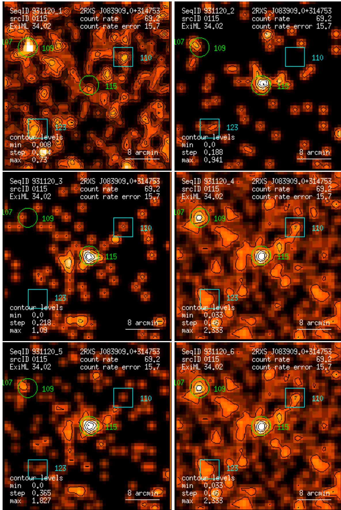
Figure 115: RASS 931120: detection 0115: band rate images, Gaussian filter: (1) PSPC channels 11 – 41, (2) 52 – 90, (3) 91 – 201, (4) 11 – 235, (5) 52 – 201, (6) 11 – 201. Broad band rates in counts/ks. Band rate contour levels in counts/ks/arcmin 2 .
