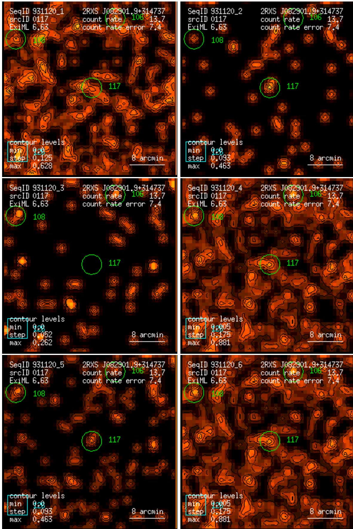
Figure 117: RASS 931120: detection 0117: band rate images, Gaussian filter: (1) PSPC channels 11 – 41, (2) 52 – 90, (3) 91 – 201, (4) 11 – 235, (5) 52 – 201, (6) 11 – 201. Broad band rates in counts/ks. Band rate contour levels in counts/ks/arcmin 2 .
