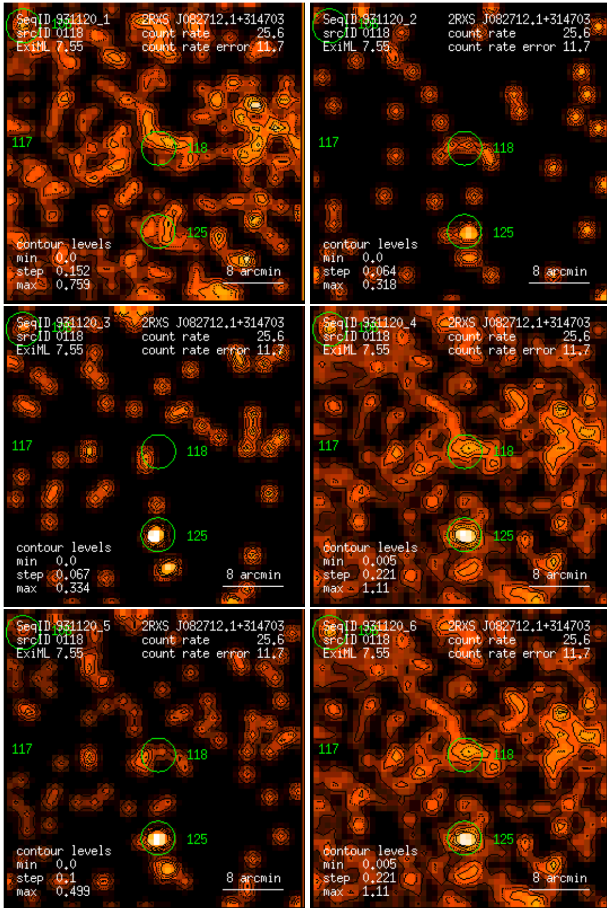
Figure 118: RASS 931120: detection 0118: band rate images, Gaussian filter: (1) PSPC channels 11 – 41, (2) 52 – 90, (3) 91 – 201, (4) 11 – 235, (5) 52 – 201, (6) 11 – 201. Broad band rates in counts/ks. Band rate contour levels in counts/ks/arcmin 2 .
