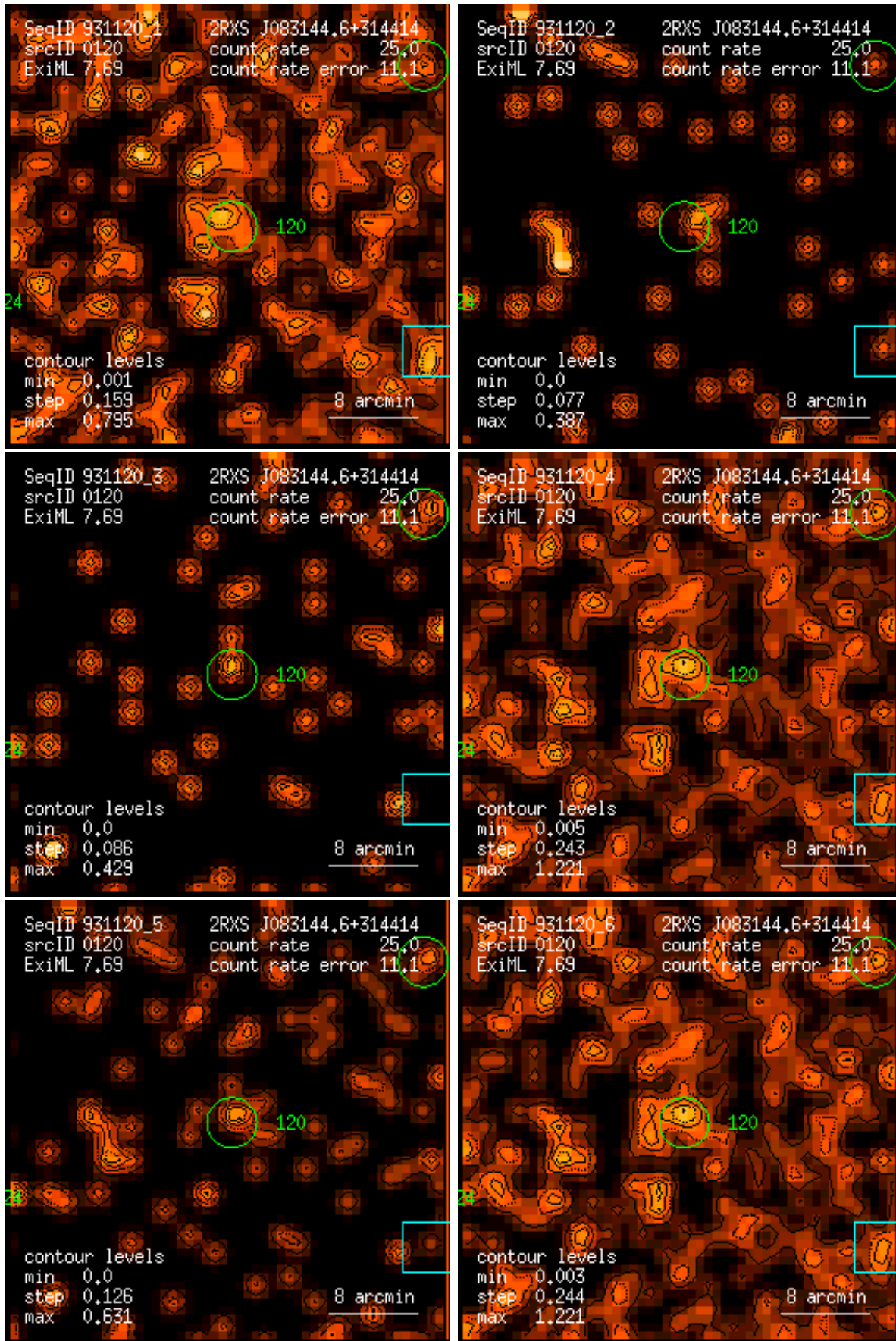
Figure 120: RASS 931120: detection 0120: band rate images, Gaussian filter: (1) PSPC channels 11 – 41, (2) 52 – 90, (3) 91 – 201, (4) 11 – 235, (5) 52 – 201, (6) 11 – 201. Broad band rates in counts/ks. Band rate contour levels in counts/ks/arcmin 2 .
