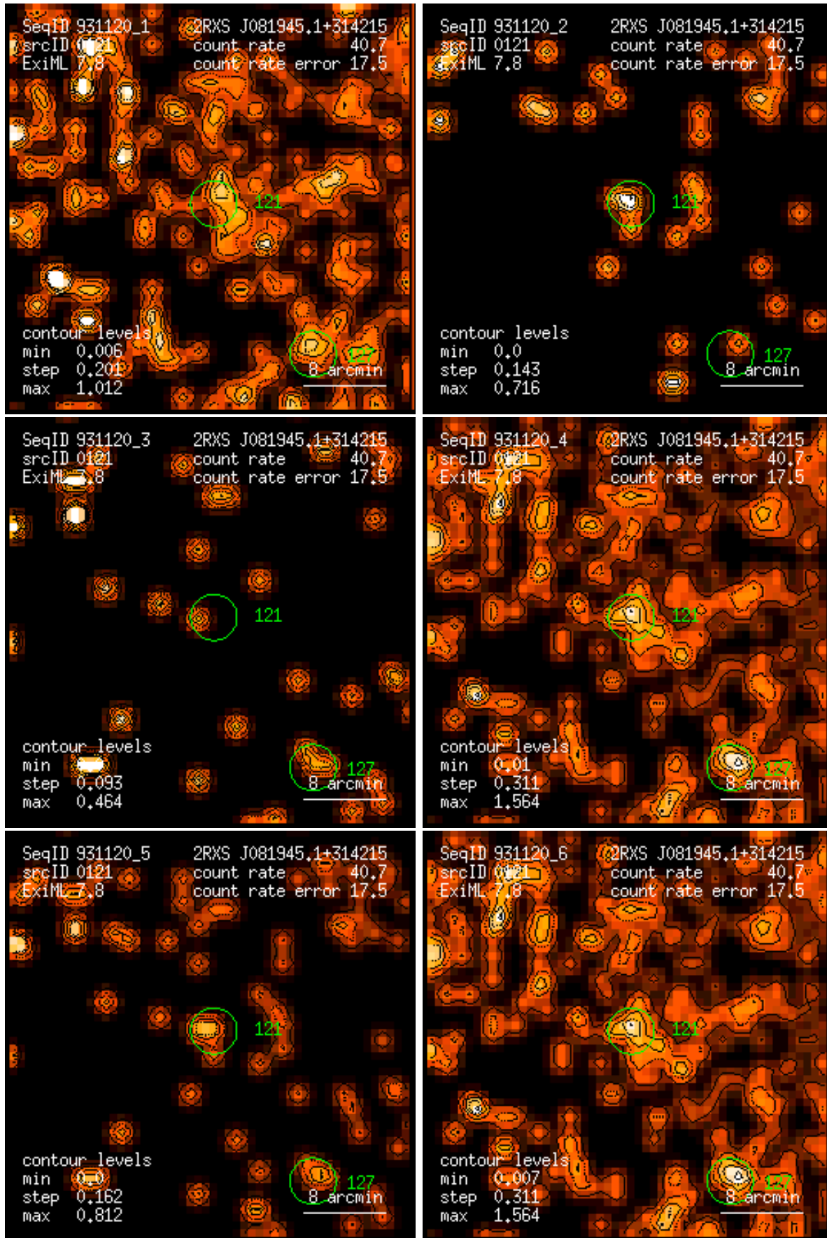
Figure 121: RASS 931120: detection 0121: band rate images, Gaussian filter: (1) PSPC channels 11 – 41, (2) 52 – 90, (3) 91 – 201, (4) 11 – 235, (5) 52 – 201, (6) 11 – 201. Broad band rates in counts/ks. Band rate contour levels in counts/ks/arcmin 2 .
