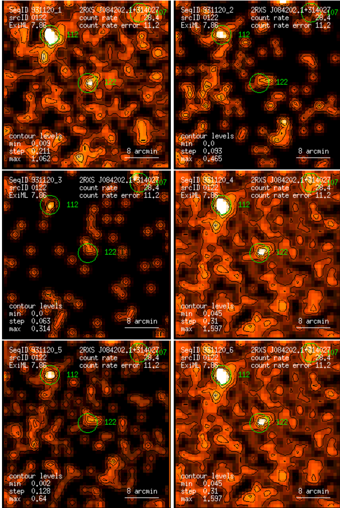
Figure 122: RASS 931120: detection 0122: band rate images, Gaussian filter: (1) PSPC channels 11 – 41, (2) 52 – 90, (3) 91 – 201, (4) 11 – 235, (5) 52 – 201, (6) 11 – 201. Broad band rates in counts/ks. Band rate contour levels in counts/ks/arcmin 2 .
