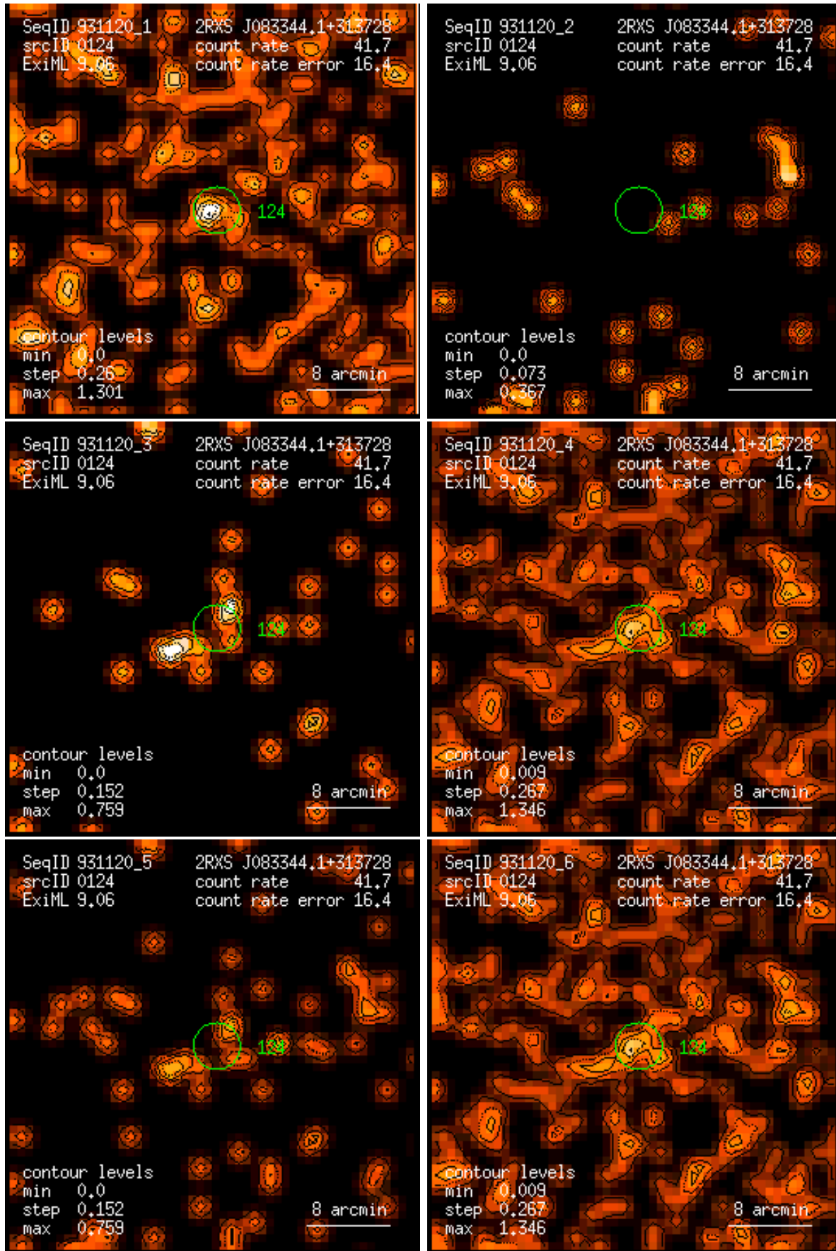
Figure 124: RASS 931120: detection 0124: band rate images, Gaussian filter: (1) PSPC channels 11 – 41, (2) 52 – 90, (3) 91 – 201, (4) 11 – 235, (5) 52 – 201, (6) 11 – 201. Broad band rates in counts/ks. Band rate contour levels in counts/ks/arcmin 2 .
