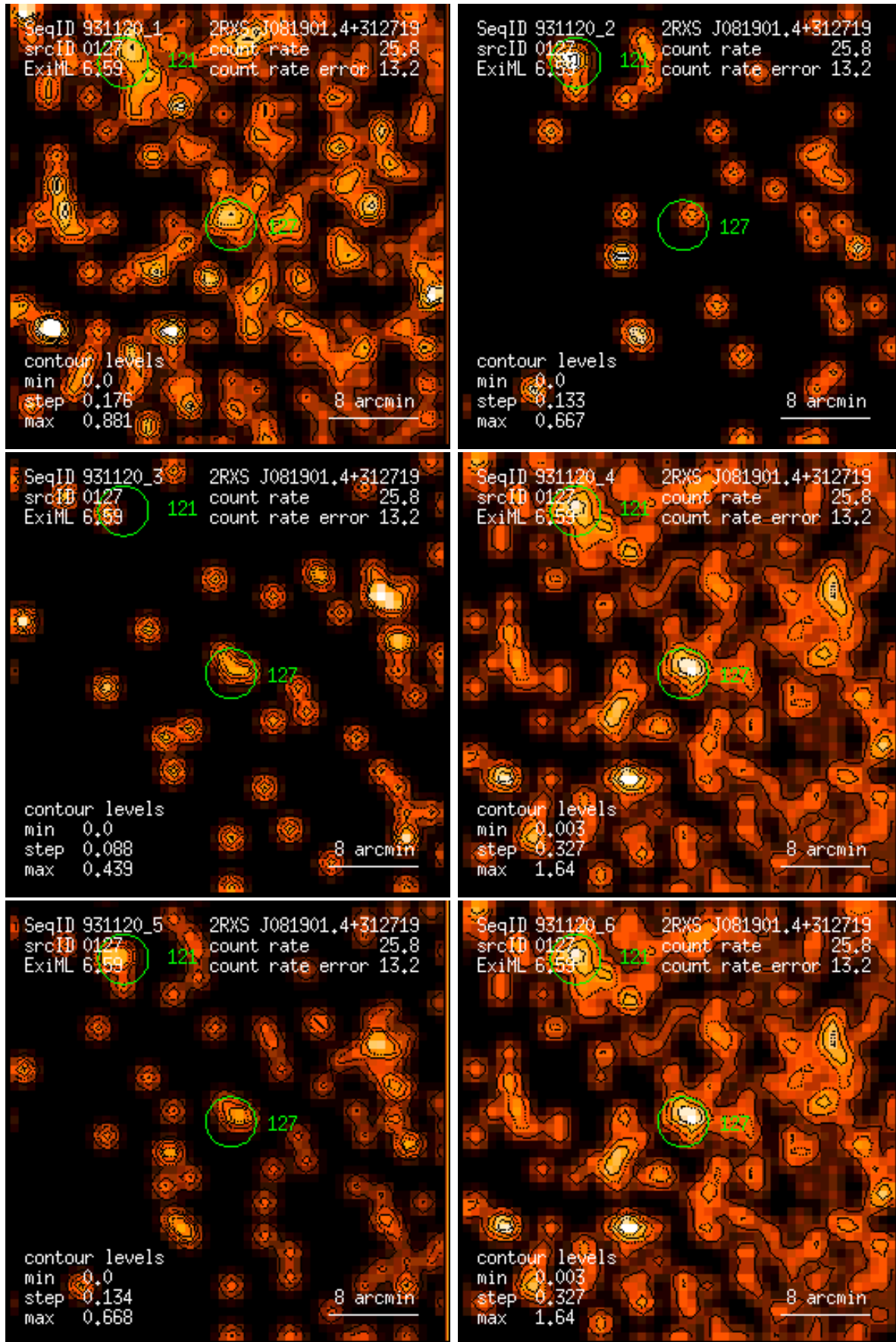
Figure 127: RASS 931120: detection 0127: band rate images, Gaussian filter: (1) PSPC channels 11 – 41, (2) 52 – 90, (3) 91 – 201, (4) 11 – 235, (5) 52 – 201, (6) 11 – 201. Broad band rates in counts/ks. Band rate contour levels in counts/ks/arcmin 2 .
