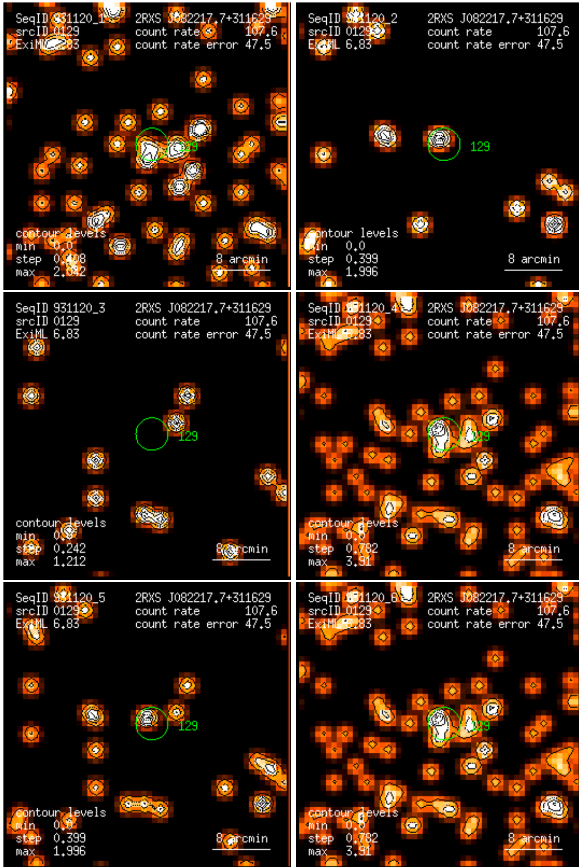
Figure 129: RASS 931120: detection 0129: band rate images, Gaussian filter: (1) PSPC channels 11 – 41, (2) 52 – 90, (3) 91 – 201, (4) 11 – 235, (5) 52 – 201, (6) 11 – 201. Broad band rates in counts/ks. Band rate contour levels in counts/ks/arcmin 2 .
