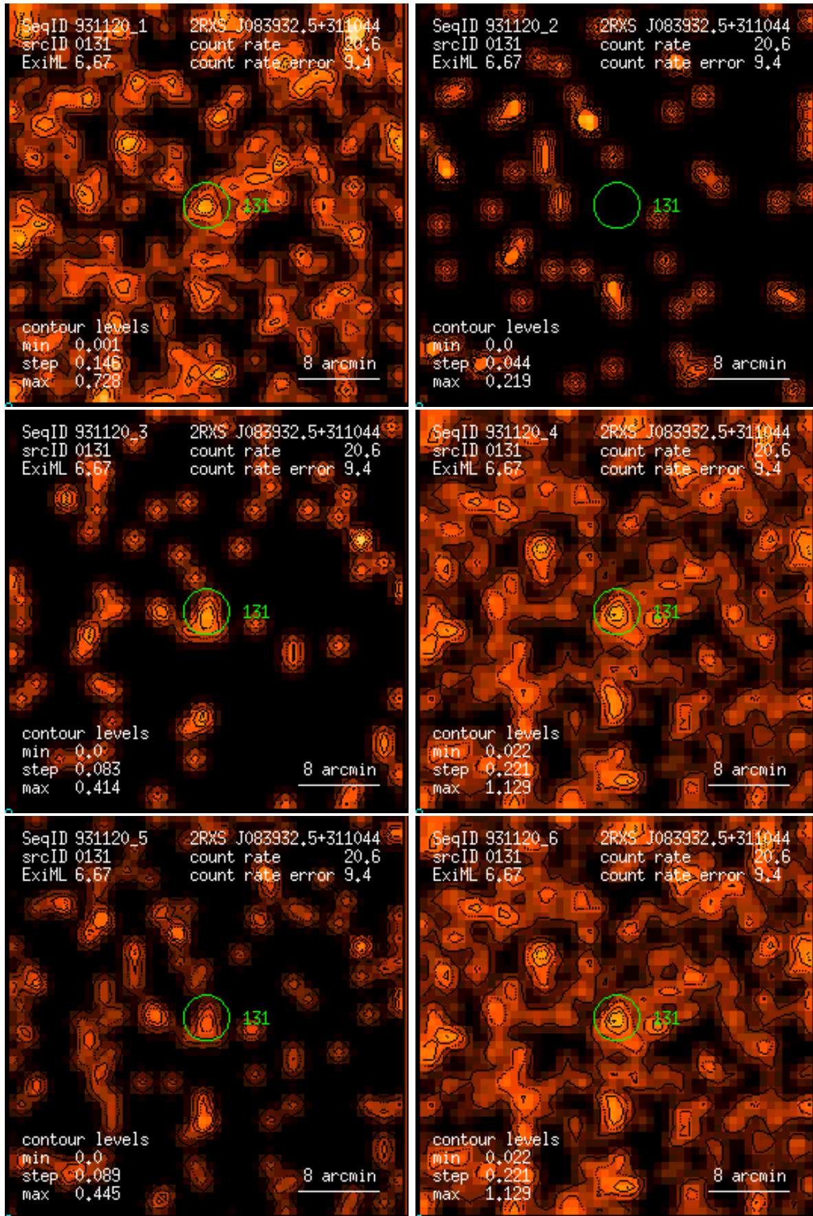
Figure 131: RASS 931120: detection 0131: band rate images, Gaussian filter: (1) PSPC channels 11 – 41, (2) 52 – 90, (3) 91 – 201, (4) 11 – 235, (5) 52 – 201, (6) 11 – 201. Broad band rates in counts/ks. Band rate contour levels in counts/ks/arcmin 2 .
