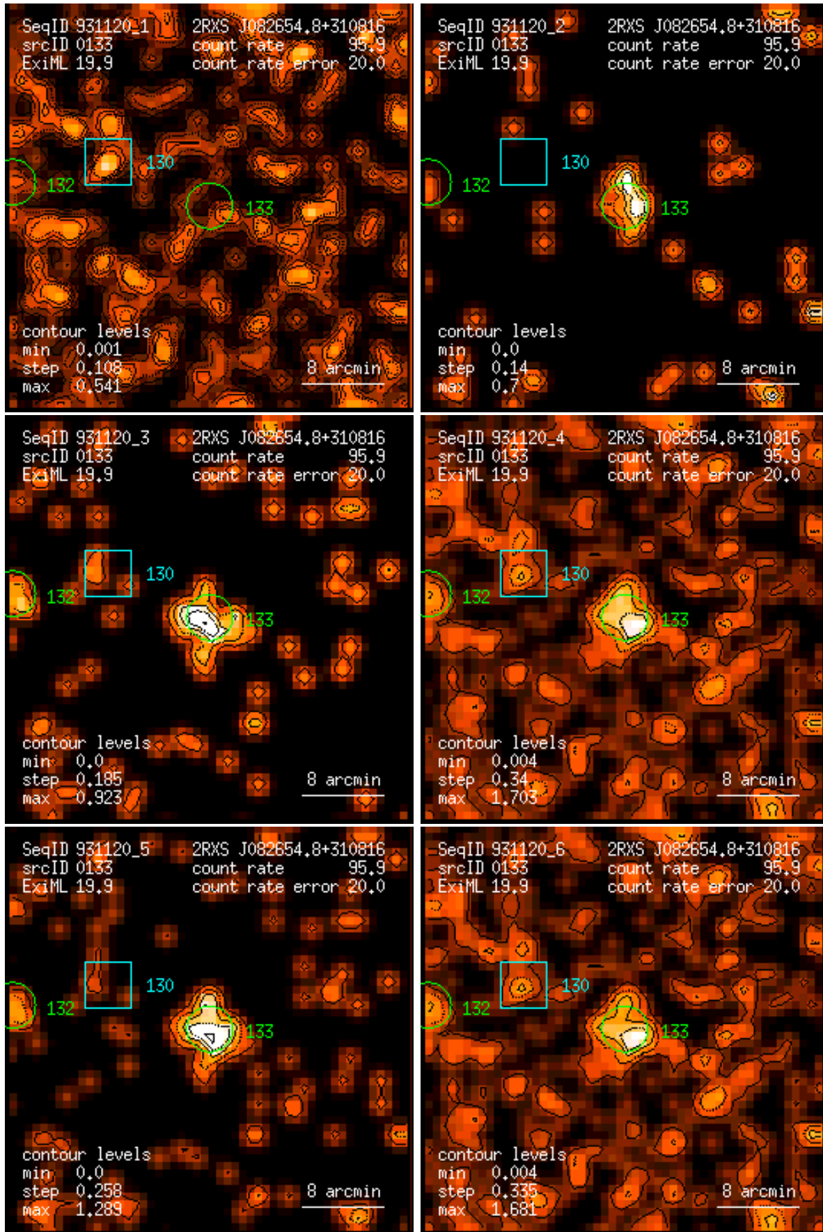
Figure 133: RASS 931120: detection 0133: band rate images, Gaussian filter: (1) PSPC channels 11 – 41, (2) 52 – 90, (3) 91 – 201, (4) 11 – 235, (5) 52 – 201, (6) 11 – 201. Broad band rates in counts/ks. Band rate contour levels in counts/ks/arcmin 2 .
