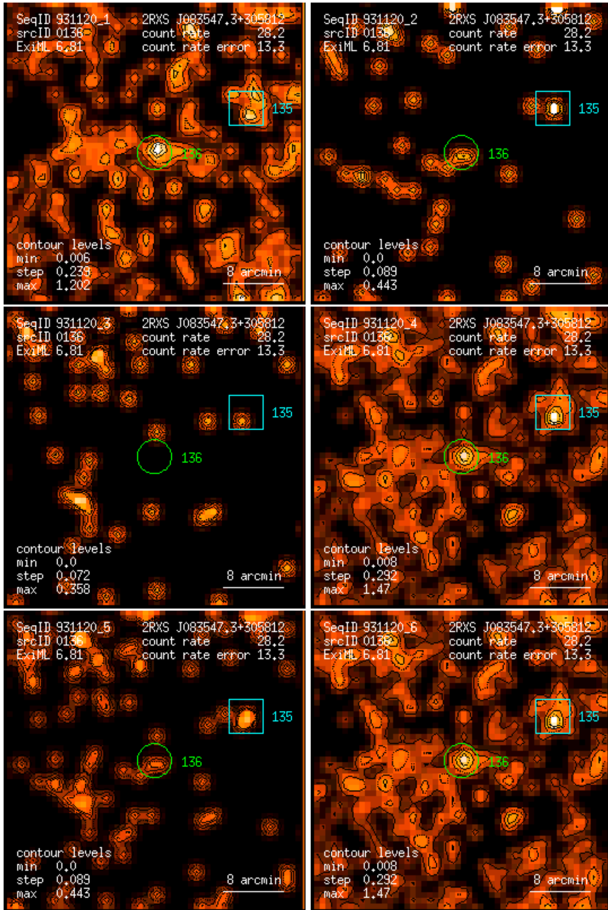
Figure 136: RASS 931120: detection 0136: band rate images, Gaussian filter: (1) PSPC channels 11 – 41, (2) 52 – 90, (3) 91 – 201, (4) 11 – 235, (5) 52 – 201, (6) 11 – 201. Broad band rates in counts/ks. Band rate contour levels in counts/ks/arcmin 2 .
