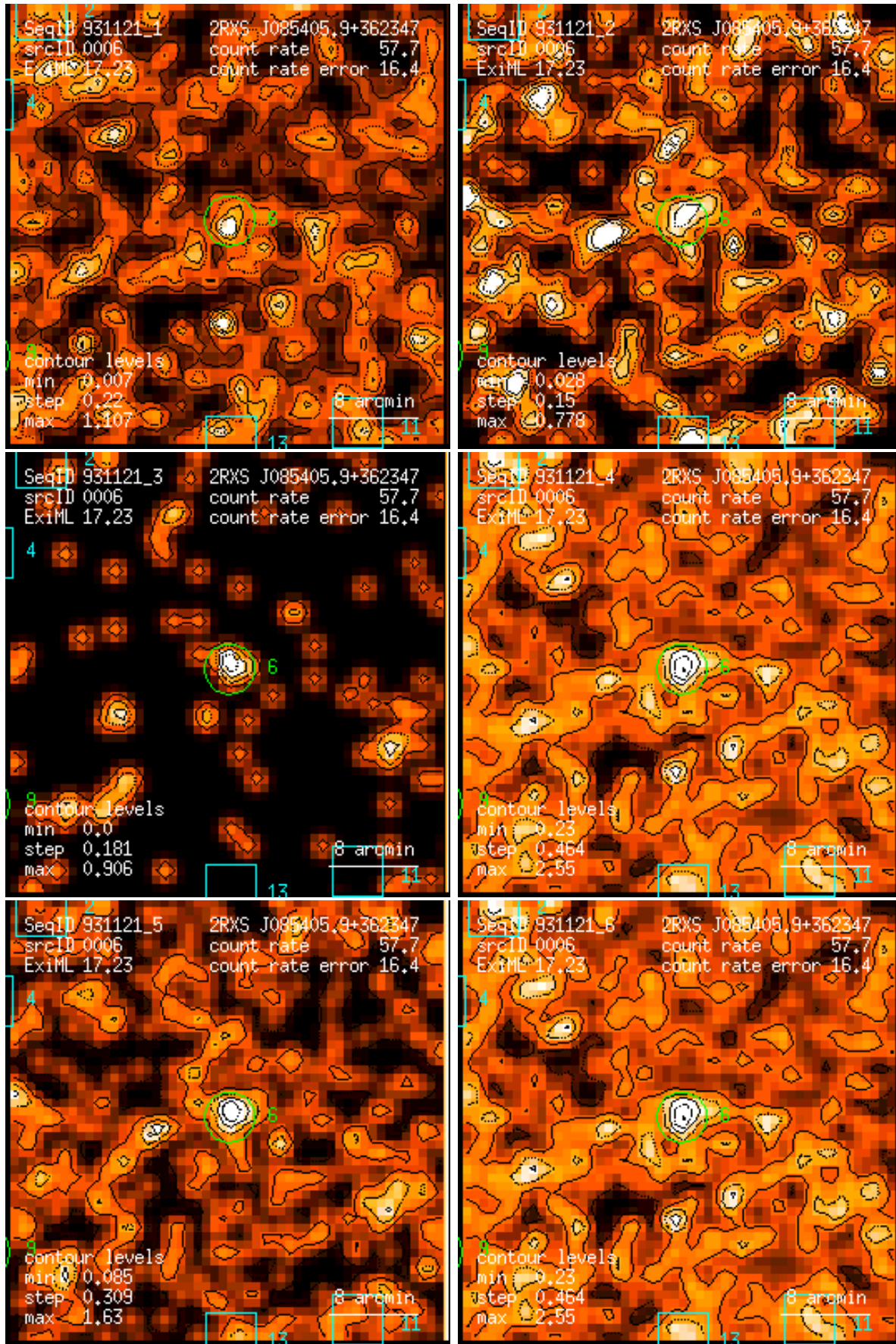
Figure 6: RASS 931121: detection 0006: band rate images, Gaussian filter: (1) PSPC channels 11 – 41, (2) 52 – 90, (3) 91 – 201, (4) 11 – 235, (5) 52 – 201, (6) 11 – 201. Broad band rates in counts/ks. Band rate contour levels in counts/ks/arcmin 2 .
