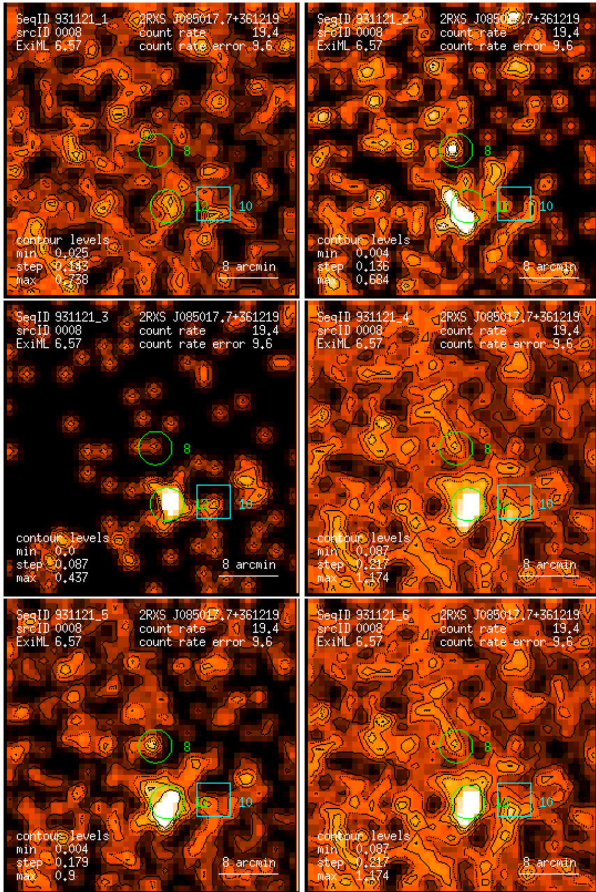
Figure 8: RASS 931121: detection 0008: band rate images, Gaussian filter: (1) PSPC channels 11 – 41, (2) 52 – 90, (3) 91 – 201, (4) 11 – 235, (5) 52 – 201, (6) 11 – 201. Broad band rates in counts/ks. Band rate contour levels in counts/ks/arcmin 2 .
