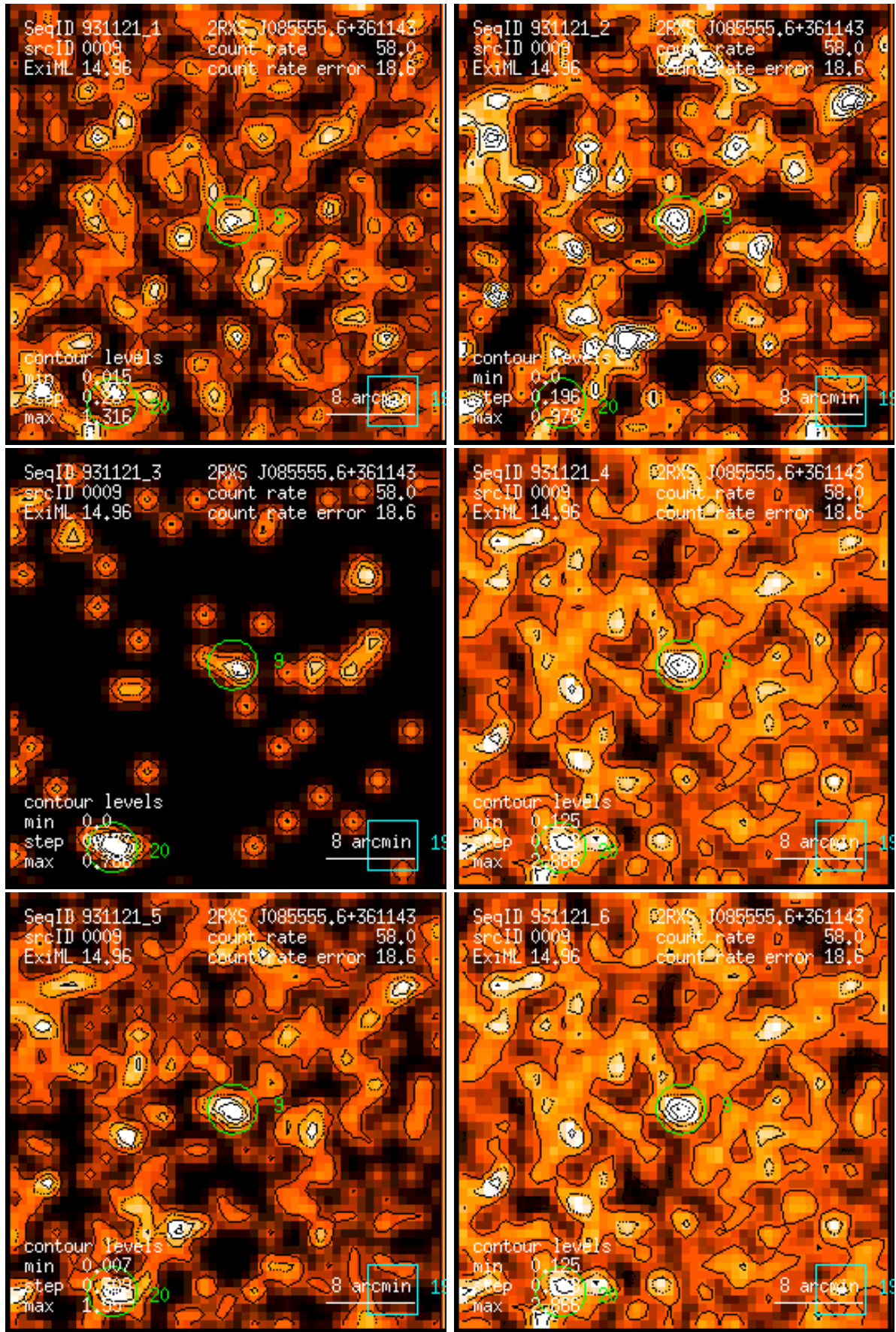
Figure 9: RASS 931121: detection 0009: band rate images, Gaussian filter: (1) PSPC channels 11 – 41, (2) 52 – 90, (3) 91 – 201, (4) 11 – 235, (5) 52 – 201, (6) 11 – 201. Broad band rates in counts/ks. Band rate contour levels in counts/ks/arcmin 2 .
