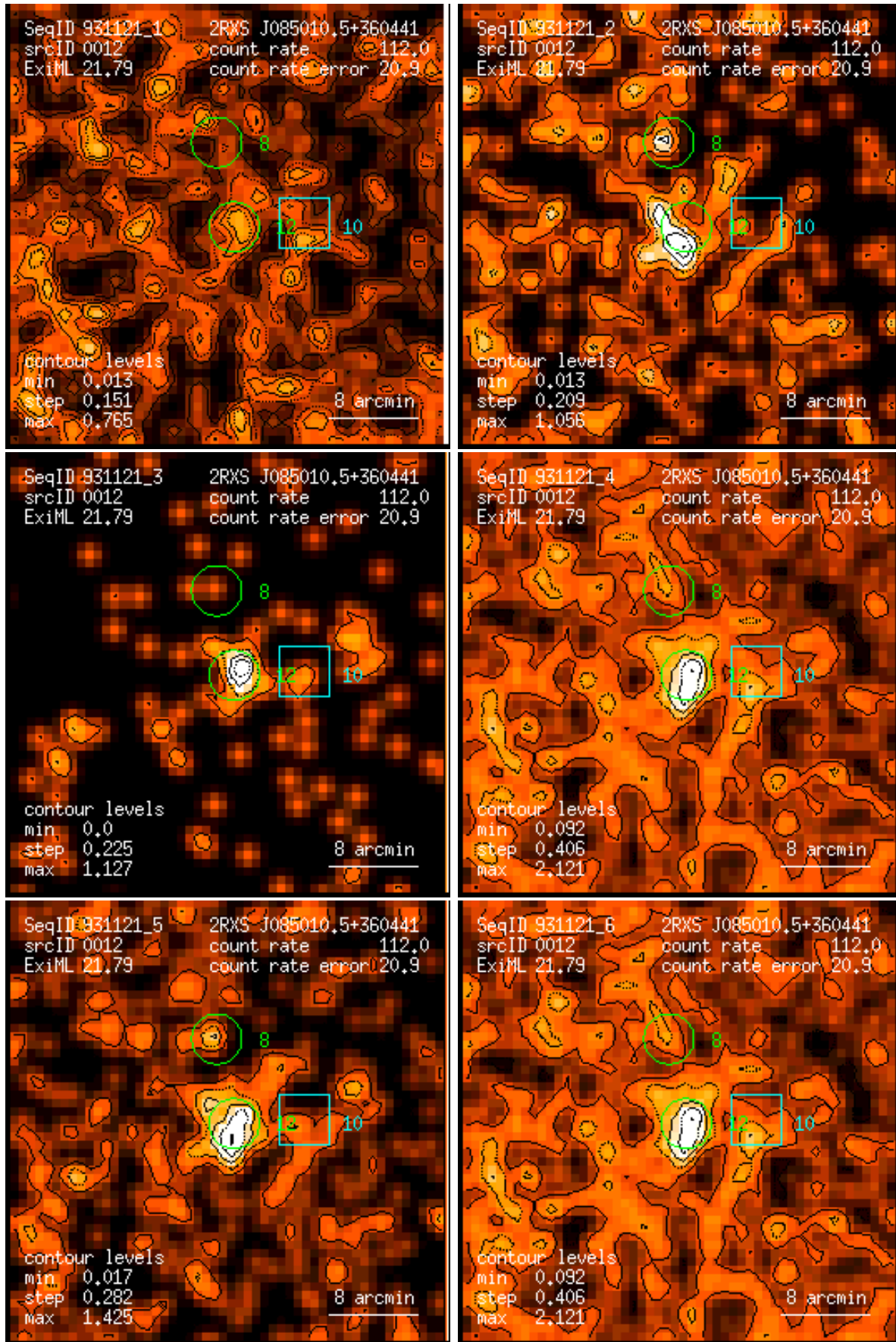
Figure 12: RASS 931121: detection 0012: band rate images, Gaussian filter: (1) PSPC channels 11 – 41, (2) 52 – 90, (3) 91 – 201, (4) 11 – 235, (5) 52 – 201, (6) 11 – 201. Broad band rates in counts/ks. Band rate contour levels in counts/ks/arcmin 2 .
