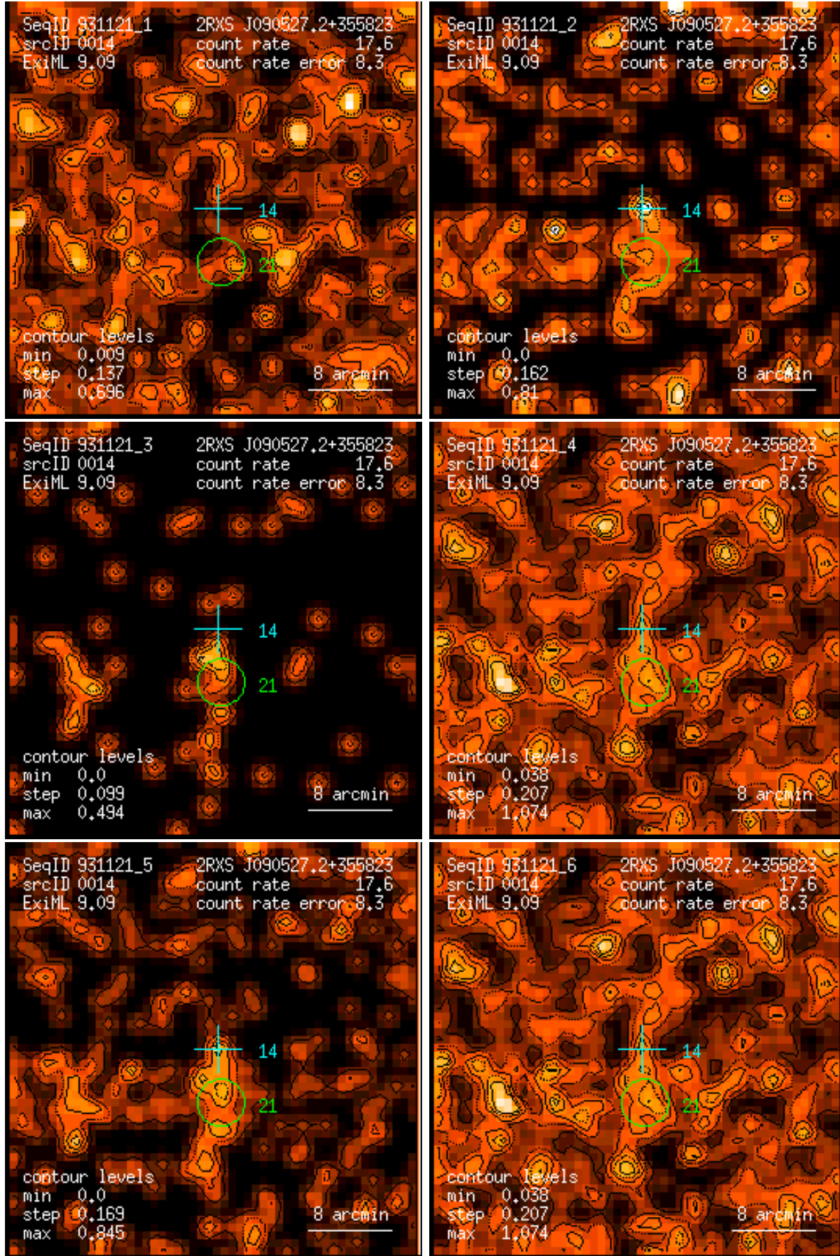
Figure 14: RASS 931121: detection 0014: band rate images, Gaussian filter: (1) PSPC channels 11 – 41, (2) 52 – 90, (3) 91 – 201, (4) 11 – 235, (5) 52 – 201, (6) 11 – 201. Broad band rates in counts/ks. Band rate contour levels in counts/ks/arcmin 2 .
