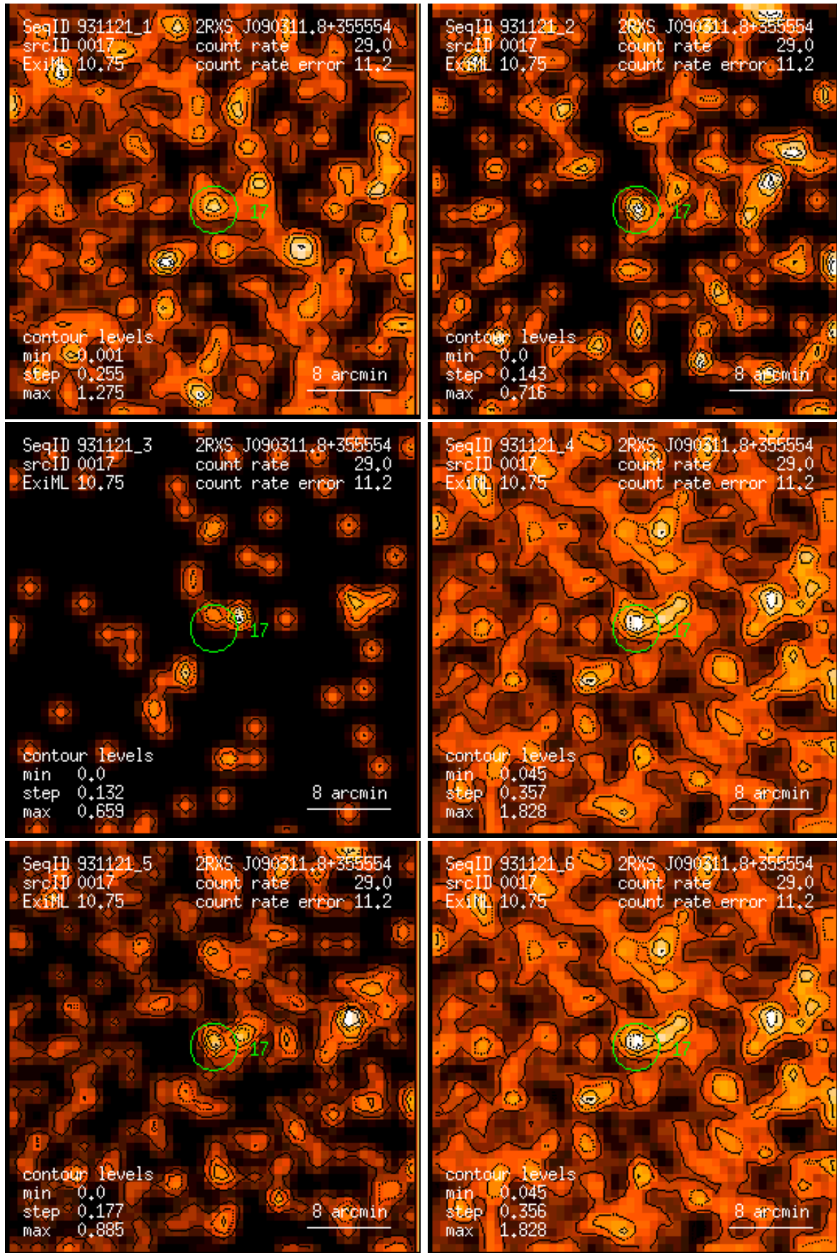
Figure 17: RASS 931121: detection 0017: band rate images, Gaussian filter: (1) PSPC channels 11 – 41, (2) 52 – 90, (3) 91 – 201, (4) 11 – 235, (5) 52 – 201, (6) 11 – 201. Broad band rates in counts/ks. Band rate contour levels in counts/ks/arcmin 2 .
