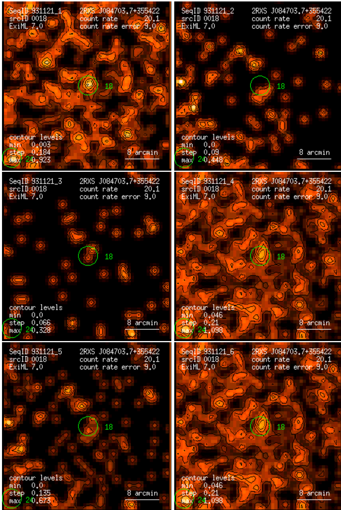
Figure 18: RASS 931121: detection 0018: band rate images, Gaussian filter: (1) PSPC channels 11 – 41, (2) 52 – 90, (3) 91 – 201, (4) 11 – 235, (5) 52 – 201, (6) 11 – 201. Broad band rates in counts/ks. Band rate contour levels in counts/ks/arcmin 2 .
