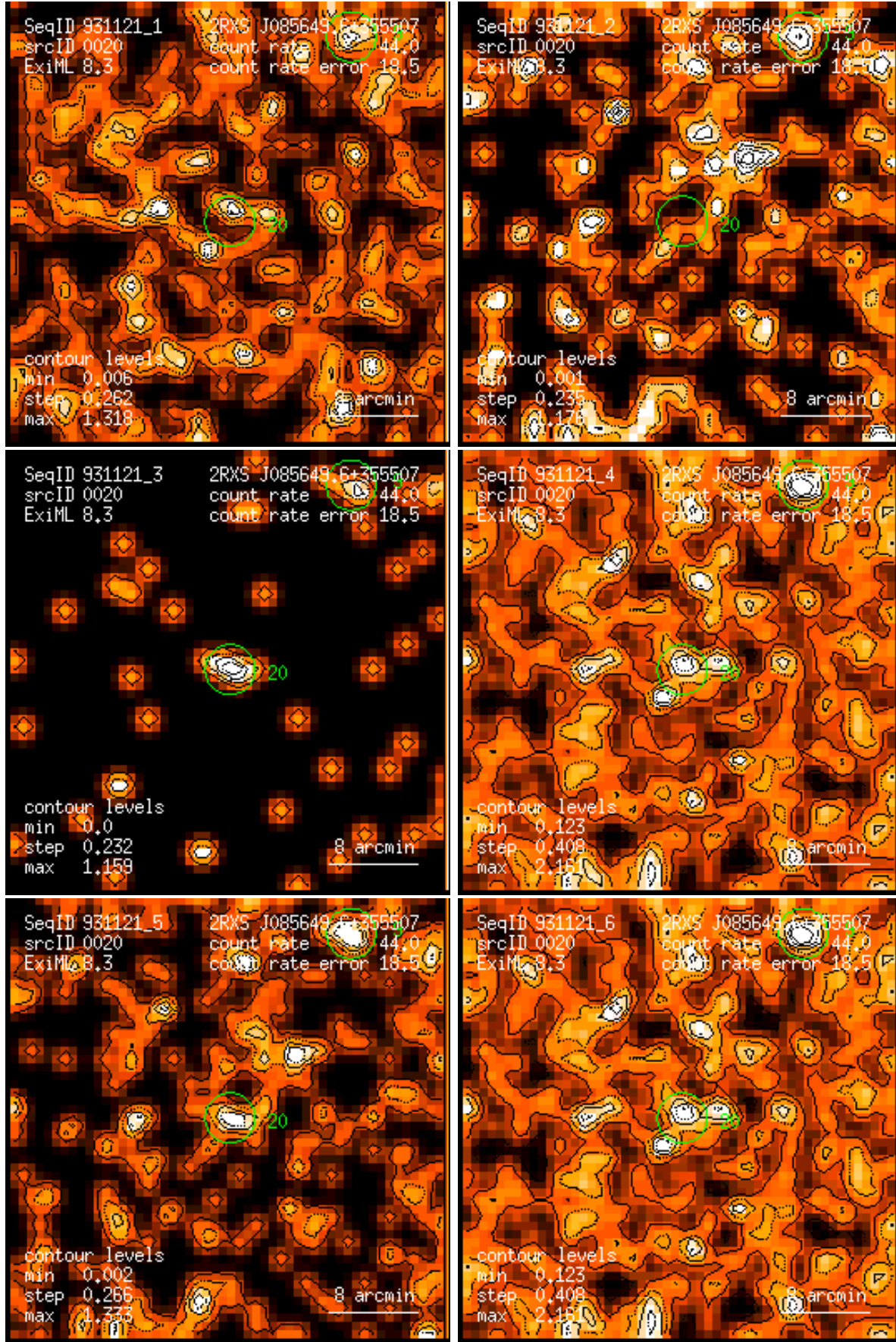
Figure 20: RASS 931121: detection 0020: band rate images, Gaussian filter: (1) PSPC channels 11 – 41, (2) 52 – 90, (3) 91 – 201, (4) 11 – 235, (5) 52 – 201, (6) 11 – 201. Broad band rates in counts/ks. Band rate contour levels in counts/ks/arcmin 2 .
