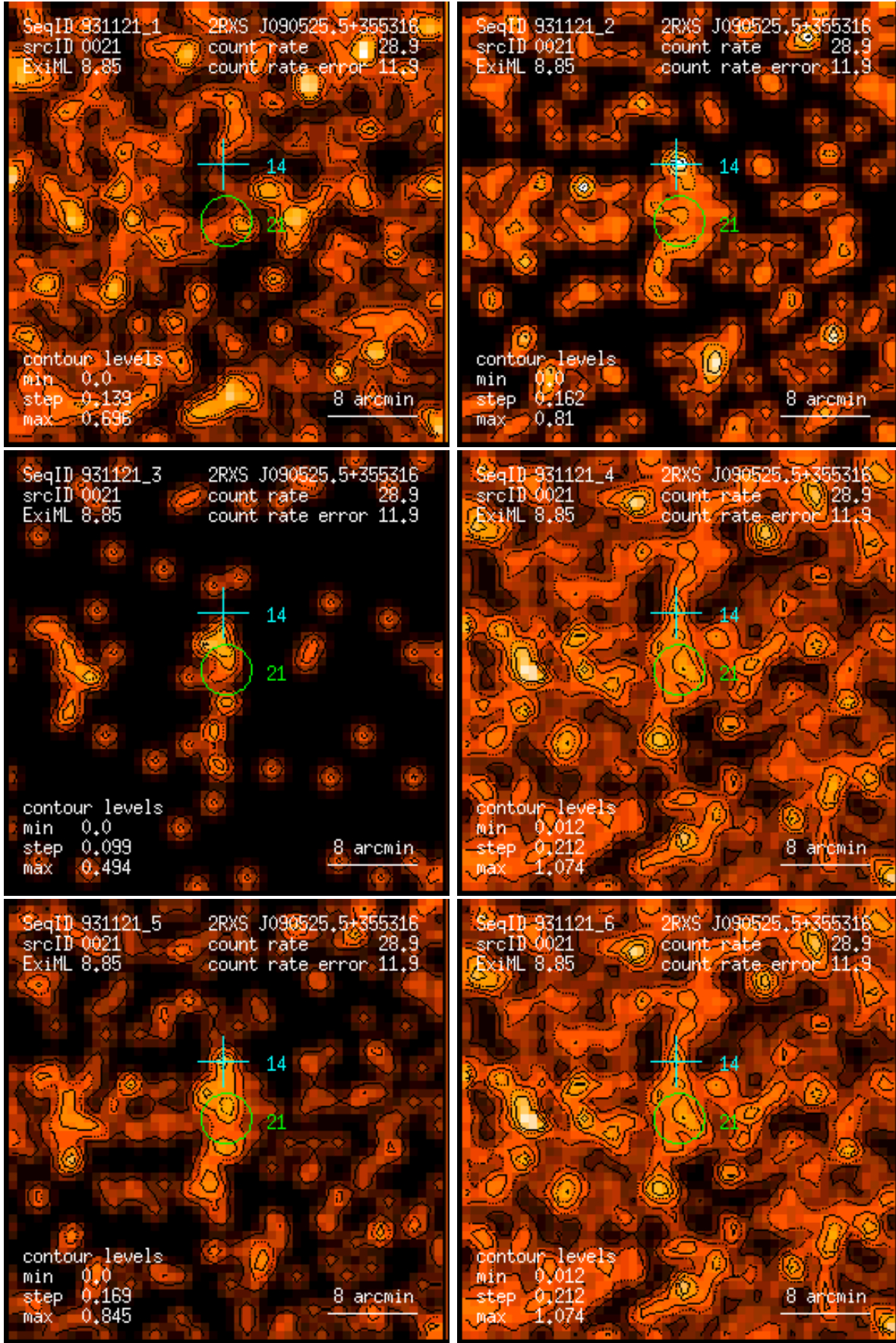
Figure 21: RASS 931121: detection 0021: band rate images, Gaussian filter: (1) PSPC channels 11 – 41, (2) 52 – 90, (3) 91 – 201, (4) 11 – 235, (5) 52 – 201, (6) 11 – 201. Broad band rates in counts/ks. Band rate contour levels in counts/ks/arcmin 2 .
