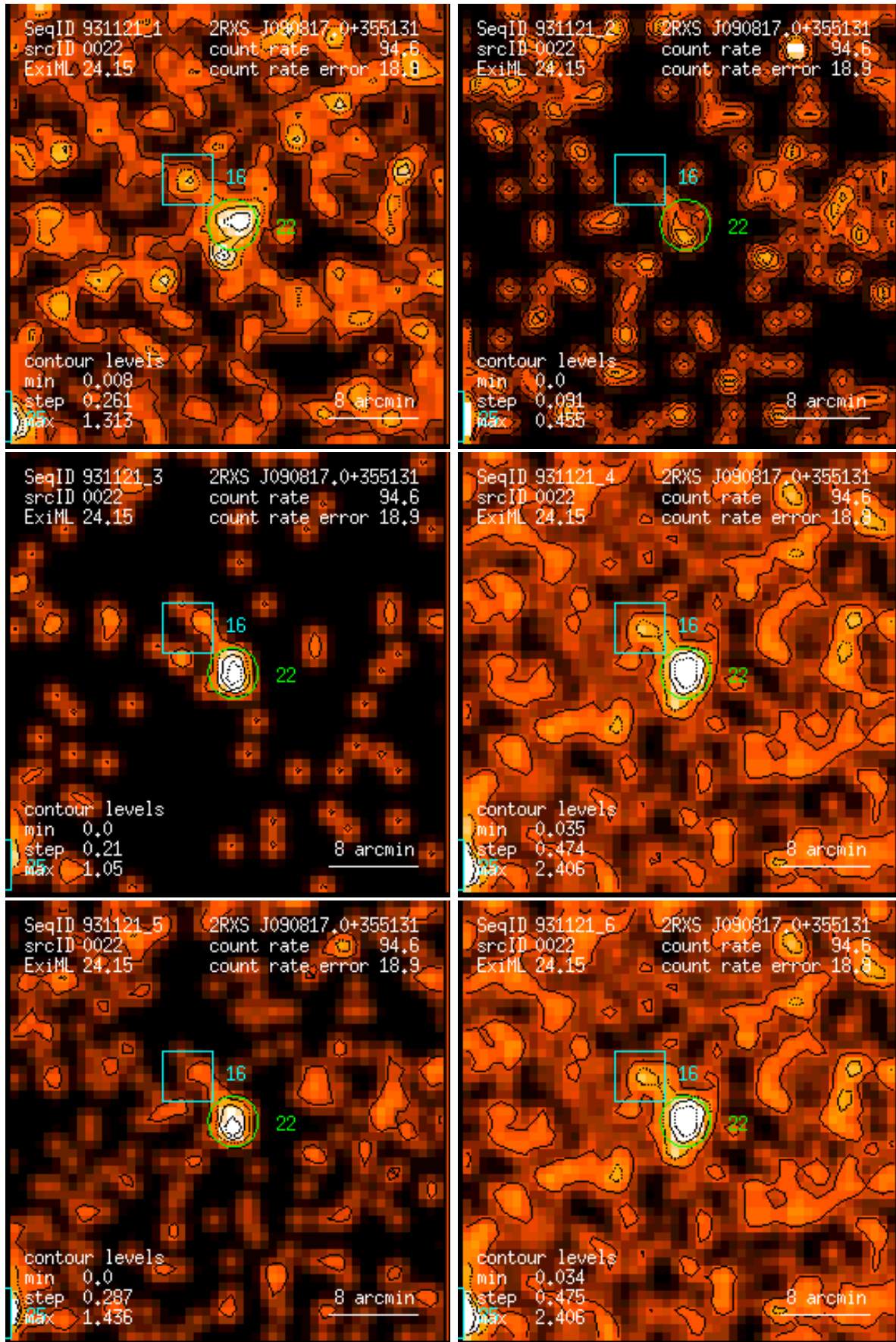
Figure 22: RASS 931121: detection 0022: band rate images, Gaussian filter: (1) PSPC channels 11 – 41, (2) 52 – 90, (3) 91 – 201, (4) 11 – 235, (5) 52 – 201, (6) 11 – 201. Broad band rates in counts/ks. Band rate contour levels in counts/ks/arcmin 2 .
